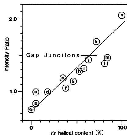
FIGURE 3 Relation of the peak intensity ratio in spherically averaged diffraction patterns to the \alpha -helical content of the protein. The ratio of average intensity in the interval 0.07\text{--}0.11\text{ \AA}^{-1} to that in the interval 0.18\text{--}0.23\text{ \AA}^{-1} is correlated with helix content of the ordered portion of the structure (those residues having an average Debye factor of <60\text{ \AA}^2 ). (a) Immunoglobulin light chain constant domain, a simple antiparallel \beta -barrel (Xu and Schiffer, 1988). (b) Plastocyanin, also a simple antiparallel \beta -barrel (Guss et al., 1986). (c) Domain 3 of TBSV coat protein, an antiparallel jellyroll \beta -barrel (Hopper et al., 1984). (d) Subtilisin inhibitor, an antiparallel \beta -sheet with transverse \alpha -helix (Mitsui et al., 1979). (e) Carboxypeptidase, an \alpha\beta mixed-sheet structure (Rees et al., 1983). (f) Flavodoxin, a parallel \beta -sheet surrounded by \alpha -helices (Smith et al., 1977). (g) Lactate dehydrogenase, structurally similar to flavodoxin (Musick and Rossman, 1979). (h) Insulin subunit, a small \alpha\beta protein in the cubic crystal form (Badger et al., manuscript in preparation). (i) Triose phosphate isomerase, a parallel \beta -barrel surrounded by \alpha -helices (Banner et al., 1976). (j) TMV coat protein, an antiparallel up-down helix bundle (Namba and Stubbs, 1986). (k) Ferricytochrome c' , an up-down divergent bundle of four antiparallel \alpha -helices (Finzel et al., 1985). (l) Hemoglobin \beta -subunit, an antiparallel helix bundle (Bolton and Perutz, 1970). (m) E. coli repressor of primer (ROP), an antiparallel up-down four-helix bundle with twofold symmetry (Banner et al., 1987). (n) Three strands of residues 96–115 from influenza virus hemagglutinin, related by a threefold axis in a parallel-stranded coiled coil (Wilson et al., 1981).
