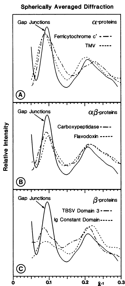
FIGURE 2 Spherically averaged intensity distributions calculated from Fourier transforms of proteins representing different structural classes. Gap junction spherically averaged diffraction, shown in each frame, was generated from the cylindrically symmetric modulated intensity (Fig. 1) by weighting each grid point by its distance R from the meridian, then integrating over all angles to the meridian. The resulting curve was low-pass Fourier filtered (with a 17\text{-}\text{\AA} resolution cutoff) and scaled with the calculated curves to have the same integrated intensity in the 4\text{--}5\text{ \AA} spacing peak. The gap junction maxima near 10\text{ \AA} falls close to curves calculated for two four-helix bundle proteins, Rhodospirillum ferricytochrome c' and tobacco mosaic virus (TMV) coat protein (A). Flavodoxin, a parallel \beta -sheet structure surrounded by \alpha -helices, and carboxypeptidase, a mixed-sheet structure surrounded by \alpha -helices, give maxima near 10\text{ \AA} smaller than that in the gap junction data (B). Antiparallel \beta -sheet structures have even smaller maxima near 10\text{ \AA} , as shown by curves calculated for tomato bushy stunt virus (TBSV) domain 3, an eight-stranded \beta -barrel, and the Bence Jones protein, an immunoglobulin constant domain \beta -barrel (C).
