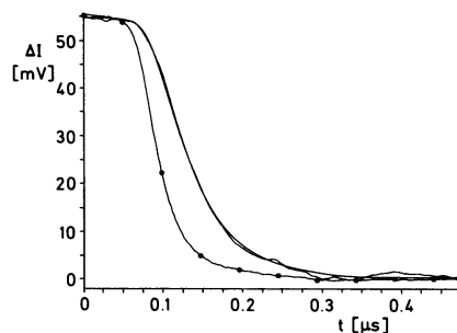
FIGURE 2 Dichroism decay curve of yeast tRNA Phe measured at 2°C in buffer B (average of 10 shots). The line marked by small circles represents the reference curve used for deconvolution and the line without noise represents a least squares fit with an exponential time constant of 39 ns. The time constants given elsewhere in the text, tables and figures were corrected for the temperature jump effect (cf. text).
