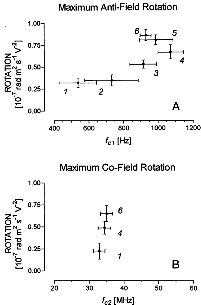
FIGURE 2 Maximum anti-field (A) and maximum co-field rotation (B) of diamide-treated platelets plotted against the first and second characteristic frequency ( f_{c1} , f_{c2} ). HEPES-Tyrode buffer, 0.5 mM diamide at 37°C; (A) (1) control, (2) 5 min, (3) 15 min, (4) 30 min, (5) 45 min, (6) 60 min, (B) (1) control, (4) 30 min, (6) 60 min. Measuring solution: 300 mOsm sucrose, 5.8 mM PBS, pH 7.2, room temperature, SE, n = 12 .
