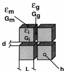
FIGURE 5 Scheme of the cubically structured model and the equivalent circuit. R and C corresponds to the resistances and capacitances of the membrane, of the cellular and the “vesicle” interior, and of the gap indicated by the indices m , i , g .
