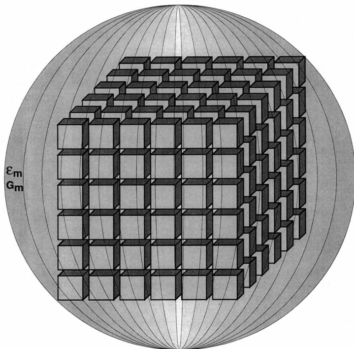
FIGURE 5 Scheme of the cubically structured model and the equivalent circuit. R and C corresponds to the resistances and capacitances of the membrane, of the cellular and the “vesicle” interior, and of the gap indicated by the indices m , i , g .
