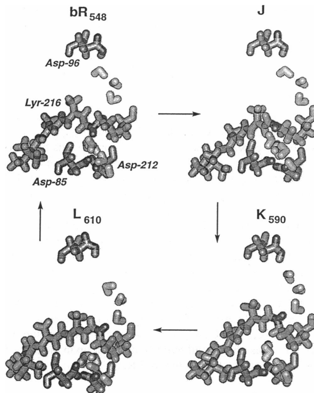
FIGURE 11 Intermediates of the 13- cis photocycle. Shown are the retinal molecule bound to a lysine side chain, three aspartic acids that play an important role in the photocycle, and the water molecules at the binding site.
