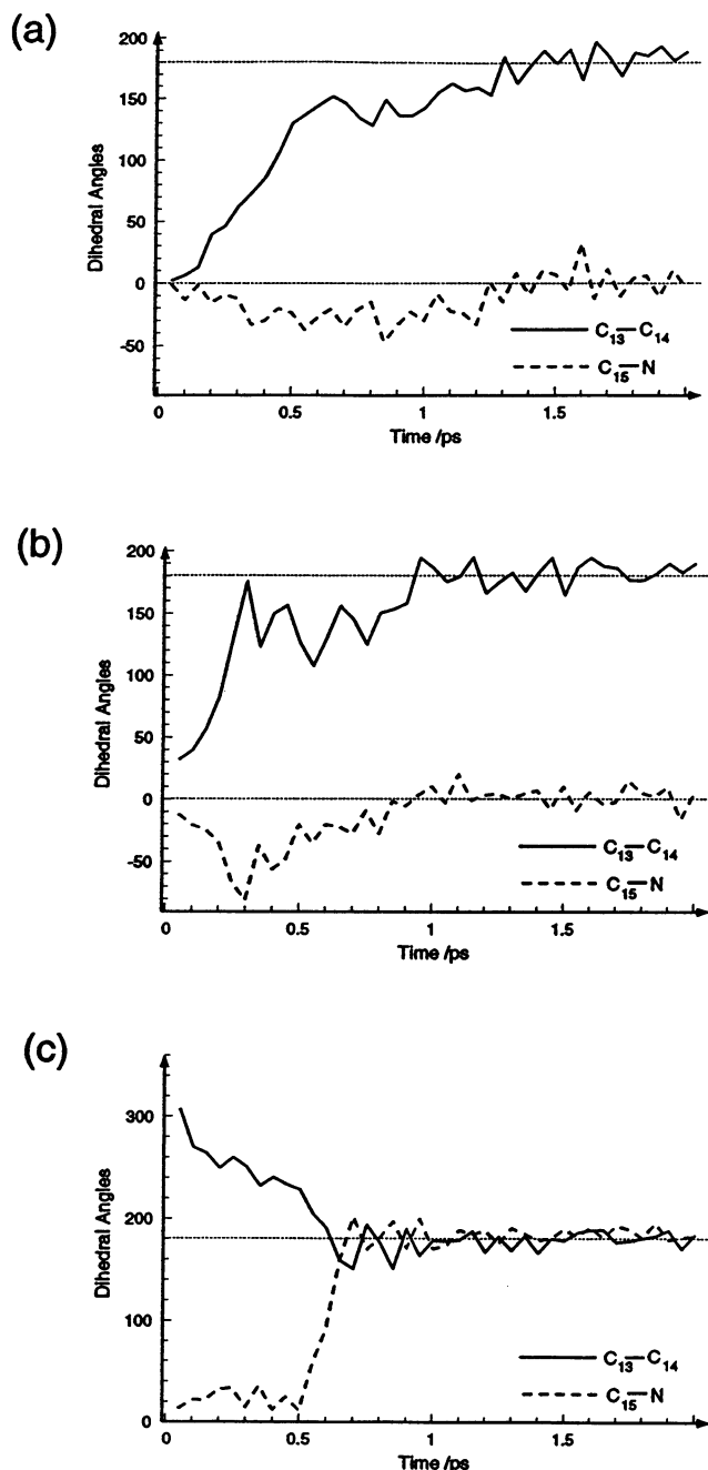
FIGURE 13 Variation of the dihedral angles of the C_{13}-C_{14} and C_{15}-N bonds of retinal during three sample cases of the photoisomerization process.
