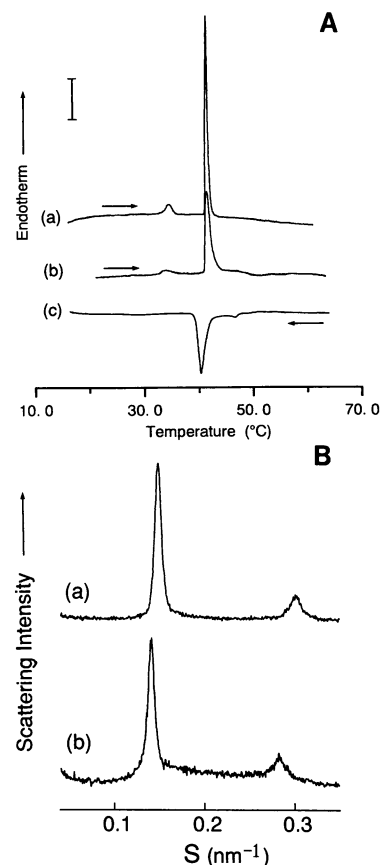
FIGURE 1 Thermal and structural parameters of aqueous dispersions of DPPC and 5 mol% DPG in DPPC. (A) Differential scanning calorimetric curves of (a) DPPC during heating at 0.8^\circ\text{C}/\text{min} , (b) heating, and (c) cooling thermograms of a mixture of DPG and DPPC at temperature rates of 0.8^\circ\text{C}/\text{min} . The bar indicates 10 kJ/mol deg. (B) Static x-ray diffraction profiles obtained from aqueous dispersions of (a) DPPC and (b) 5 mol% DPG in DPPC recorded at 42.5^\circ\text{C} .
