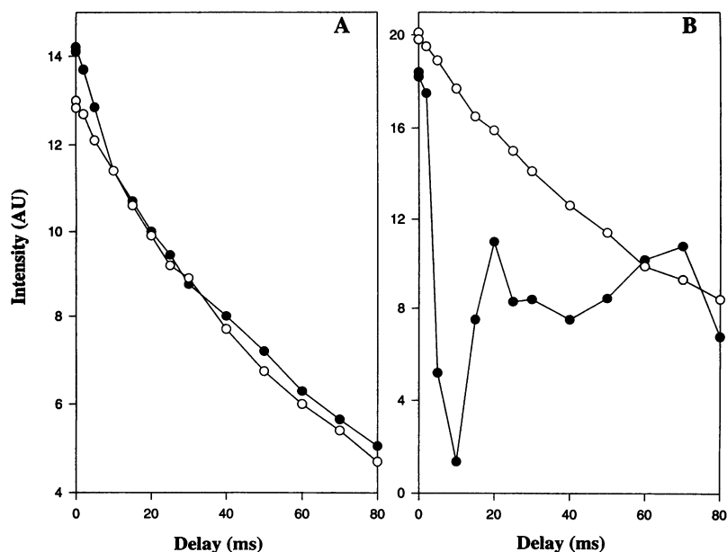
FIGURE 3 Magnetization decay of (A) the methylene choline C\beta and (B) the acyl chain methylenes C4-C11 in pure DMPC multilamellar dispersions as a function of the delay time in the HT_{1\rho} measurement experiments performed by using conventional CP (●) and RAMP-CP (○).
