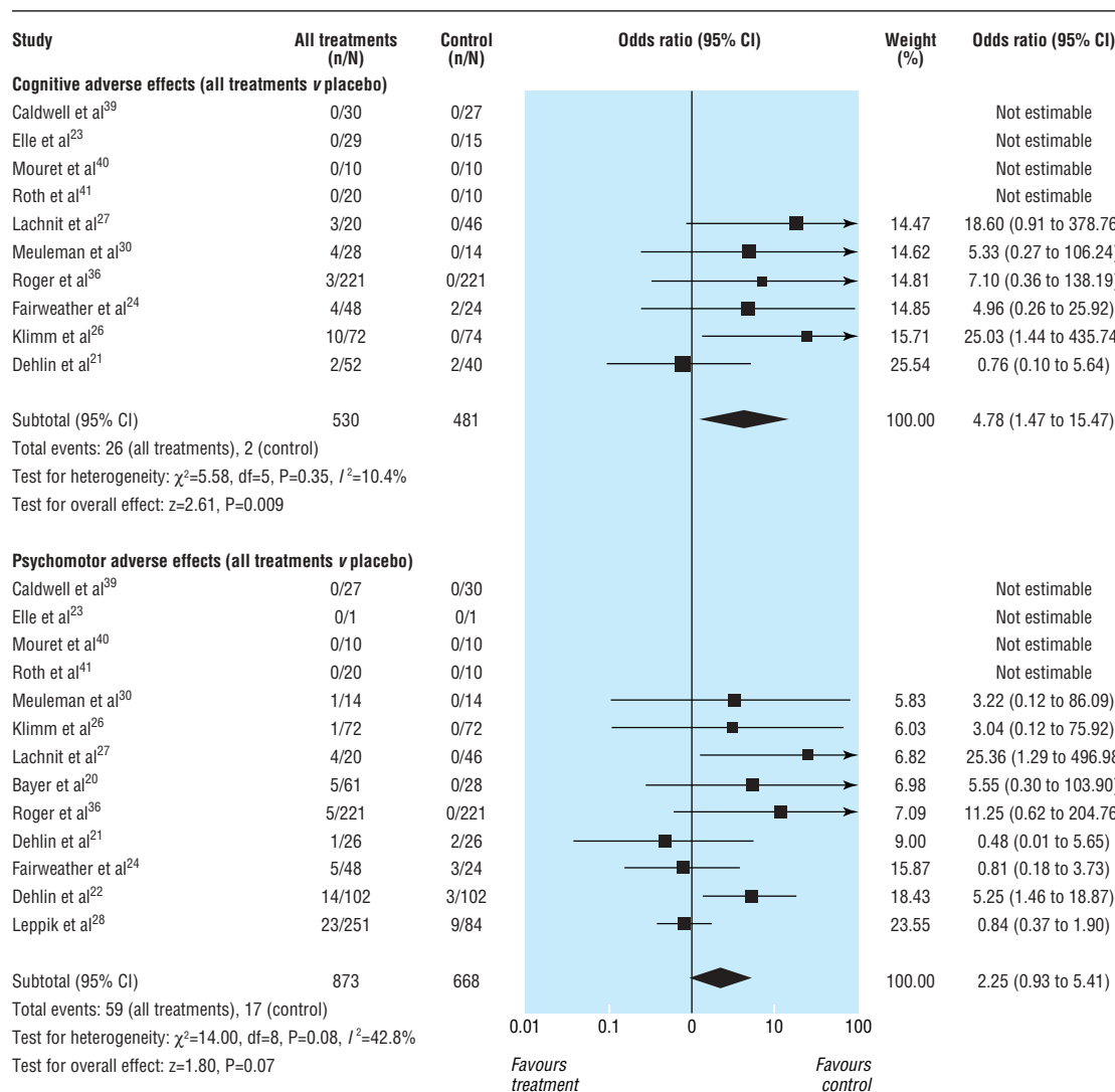
Fig 3 Cognitive and psychomotor adverse events, odds ratios, z scores, and test for heterogeneity for any sedative hypnotics taken for at least five nights in people aged 60 or older with insomnia
