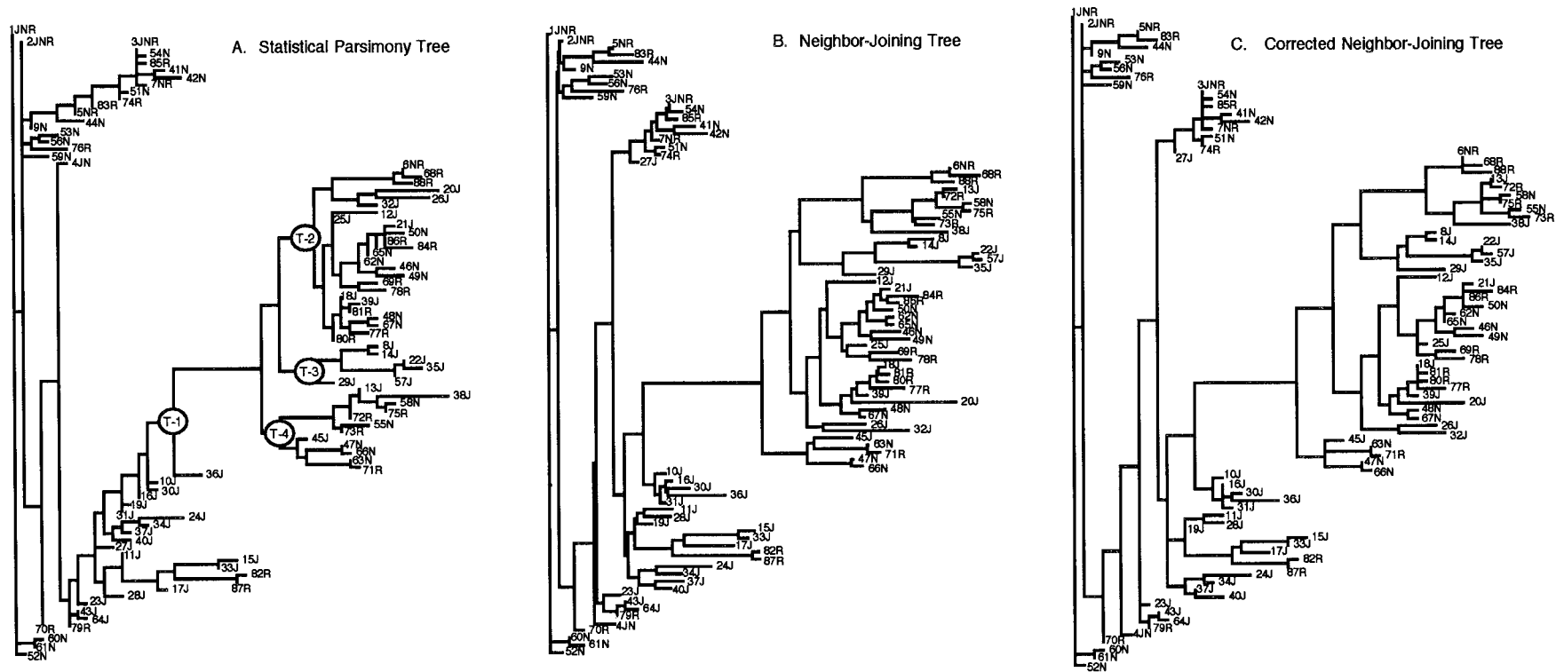
Figure 1 Evolutionary “trees” of LPL, as estimated by three procedures. In each case, only the horizontal length of branches indicate mutational change, with the length proportional to the number of mutations on that branch. Haplotypes are indicated by a number, followed by one or more letters indicating the populations in which that particular haplotype was present (J = Jackson, N = North Karelia, and R = Rochester). A, Statistical parsimony “tree.” Nodes that define four major clades are indicated by an oval containing “T-i,” where i can be 1, 2, 3, or 4. There are actually 8 “trees” in the statistically parsimonious confidence set, but the differences from the one portrayed here are minor. The full set of SP trees is available at the MDECODE Web site. B, NJ “tree.” C, Corrected NJ “tree.”
