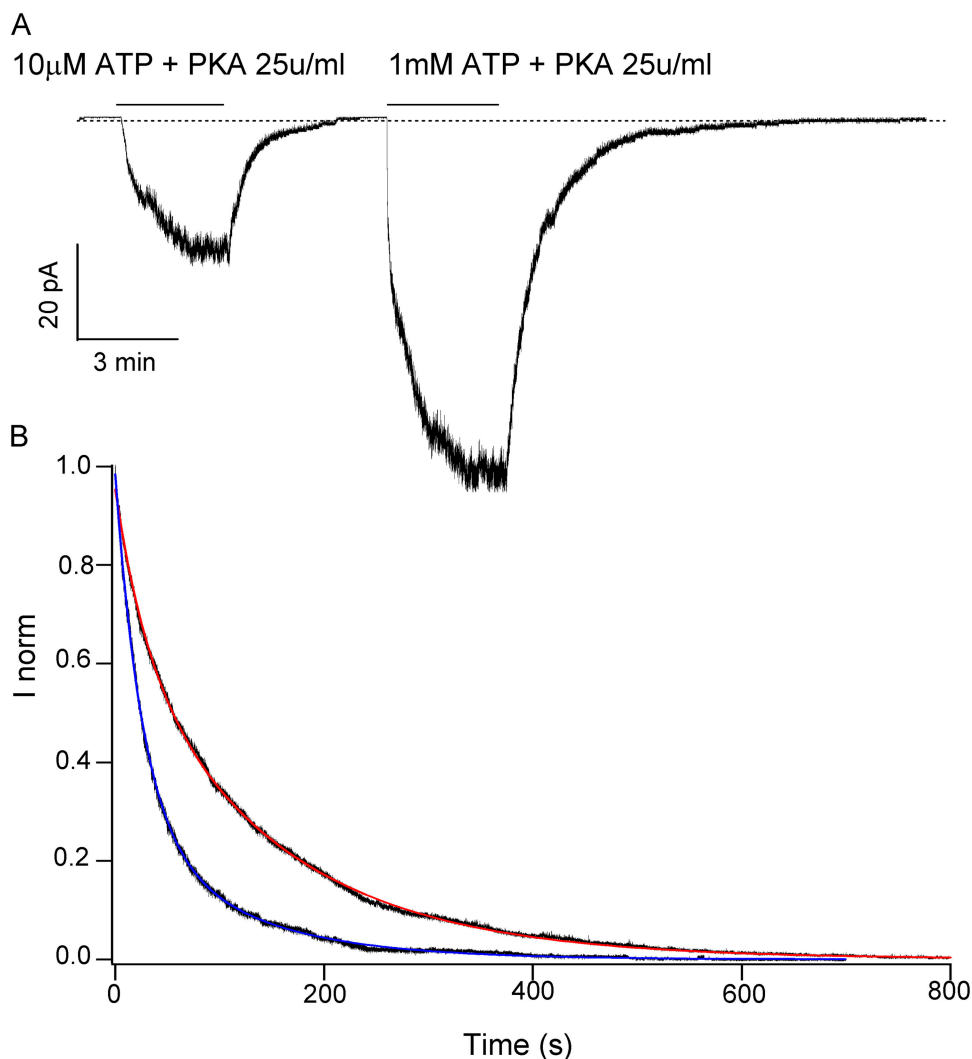
FIGURE 8. Macroscopic current relaxation of E1371S-CFTR currents. (A) Sample trace of current relaxations for E1371S-CFTR channels activated with 10 \mu M ATP + PKA, or with 1 mM ATP + PKA. (B) Normalized ensemble current relaxations upon removal of 1 mM ATP (from 12 patches) or 10 \mu M ATP (from 9 patches). The 1 mM ATP relaxation curve can be fitted with a double exponential function (red curve) with time constants of 149.3 \pm 0.02 s (69%) and 29.59 \pm 0.02 s (31%). The 10 \mu M ATP curve can be fitted also with a double exponential function (blue curve) with time constants of 107.53 \pm 0.08 s (29%), and 26.32 \pm 0.01 s (71%).
