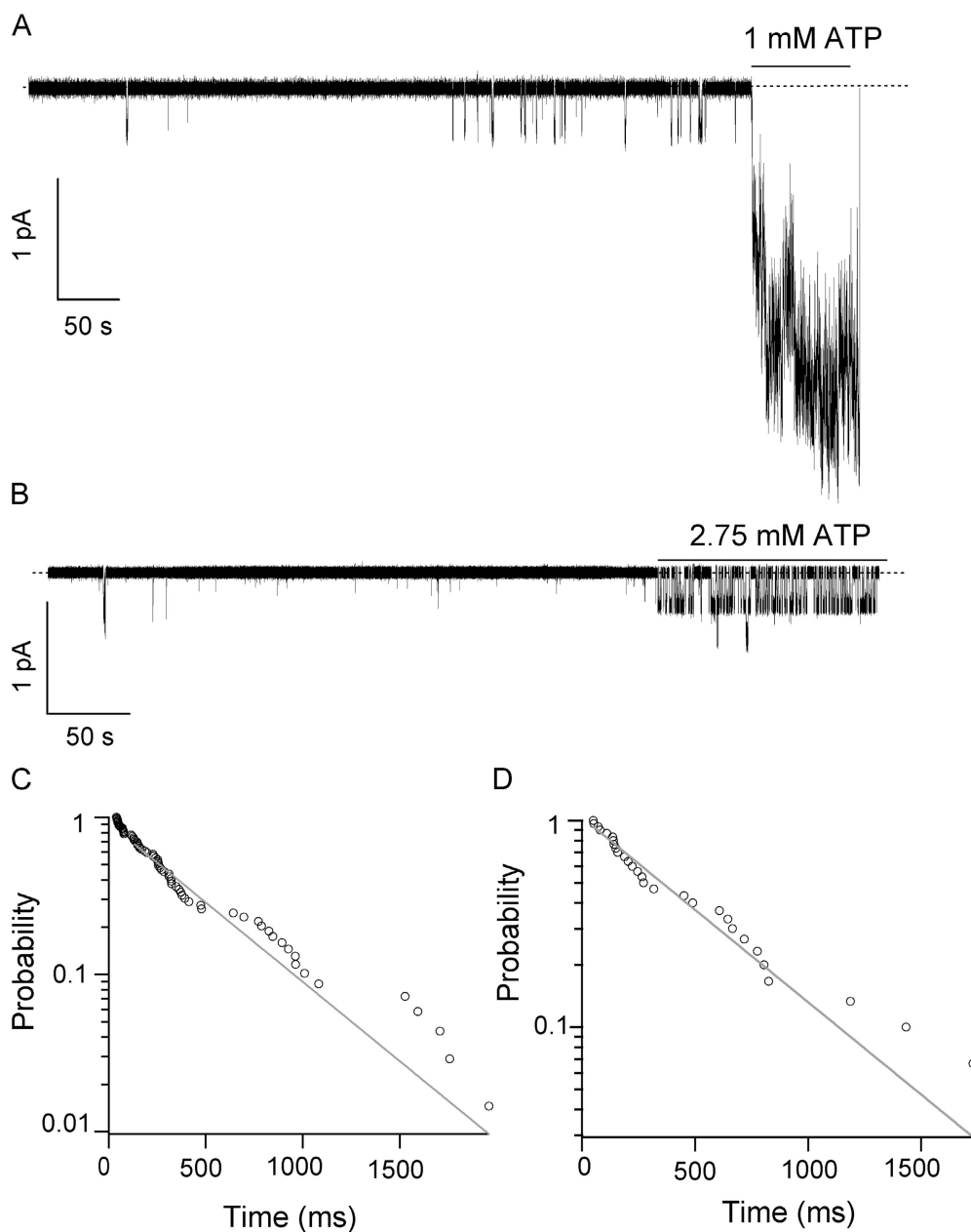
FIGURE 11. Kinetic analysis of the spontaneous openings in the absence of ATP. (A) A representative \Delta R/E1371S -CFTR current trace from an excised inside-out patch exposed to ATP-free solution for several minutes before 1 mM ATP was applied. (B) Similar experiment as described in A, but with \Delta R -CFTR channels. The open times of these spontaneous openings from several patches containing \Delta R/E1371S -CFTR (C) or \Delta R -CFTR (D) were pooled together to construct survivor plots.
