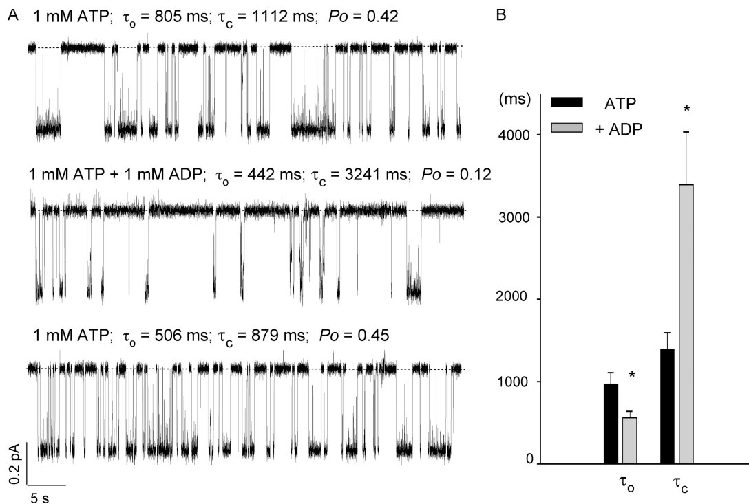
FIGURE 1. ADP shortens the open time of \Delta R/D1370N -CFTR channels. (A) Single-channel current traces in the presence of 1 mM ATP, 1 mM ATP + 1 mM ADP, or 1 mM ATP again. (B) Effects of ADP on the mean open and closed times. Notice that ADP shortens the mean open time and increases the mean closed time ( n = 5 ). Error bars represent SEM. * indicates P < 0.01 .
