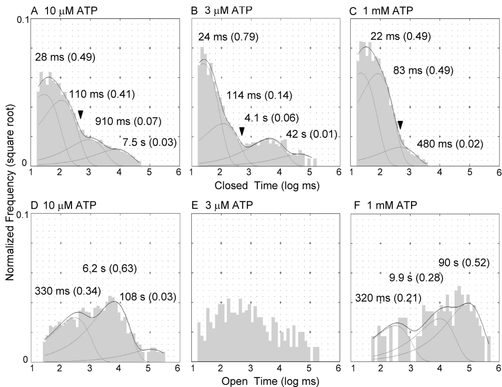
FIGURE 6. Single-channel dwell time analysis of \Delta R/E1371S -CFTR. (A) Events from two single-channel recordings ( \sim 50 min each) were pooled together to construct this closed time histogram. The closed time distribution for data obtained at 10 \mu\text{M} ATP can be fitted with a quadruple exponential function. No cutoff was used for the construction of this histogram. The arrow marks the cutoff (500 ms) used to define the minimum of the ATP-dependent closed times used for the open time analysis in D. (B) The closed time distribution for data obtained at 3 \mu\text{M} ATP and fitting parameters. (C) Events from two recordings of single channels in the presence of 1 \text{ mM} ATP were pooled together to construct this closed time histogram ( \sim 100 min of recording). The closed time distribution can be fitted with a triple expo-
