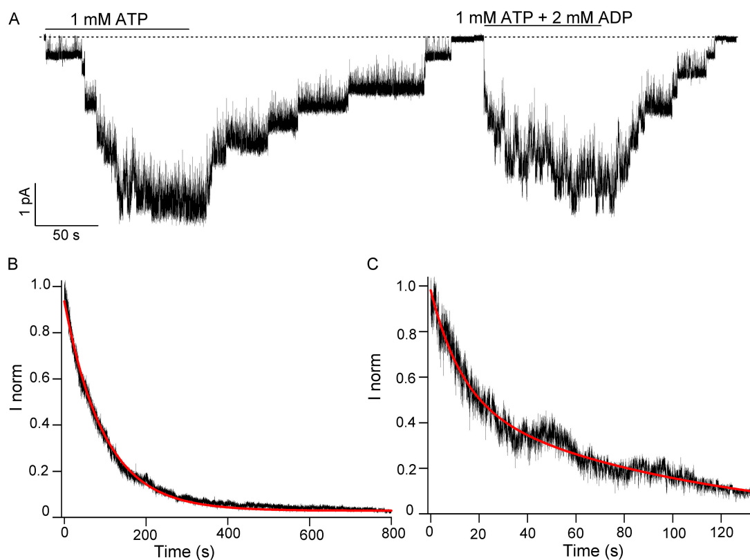
FIGURE 2. Macroscopic current relaxation for \Delta R/E1371S -CFTR channels in the presence of ATP and ADP. (A) A sample trace of current relaxations for \Delta R/E1371S -CFTR channels opened with 1 mM ATP, and subsequently with 1 mM ATP + 2 mM ADP. (B) The current decay upon removal of ATP can be fitted with a single exponential function with a time constant of 100.00 \pm 0.02 s. (C) The current decay upon removal of ATP plus ADP is fitted with a double exponential function with time constants of 12.9 \pm 0.1 and 105 \pm 3 s.
