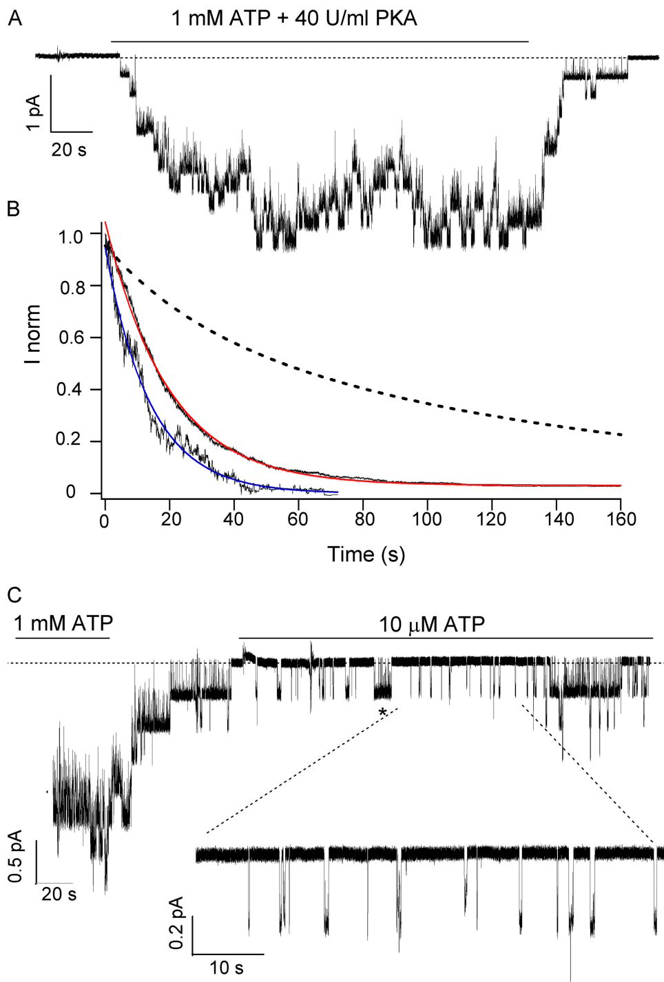
FIGURE 10. The K464A mutation shortens the locked-open time of E1371S-CFTR. (A) Sample trace of K464A/E1371S-CFTR channels in the presence of 1 mM ATP + PKA. Note that the relaxation upon nucleotide washout is very fast. (B) Ensemble macroscopic currents were generated from 18 patches. The macroscopic current has a relaxation time constant of 19.60 \pm 0.01 s (red curve). (C) Sample trace of K464A/E1371S-CFTR channels in the presence of 10 \mu M ATP (blue curve). The inset shows the presence of numerous brief openings (from 42 to 650 ms). Note also the presence of longer openings (*, 9 s).
