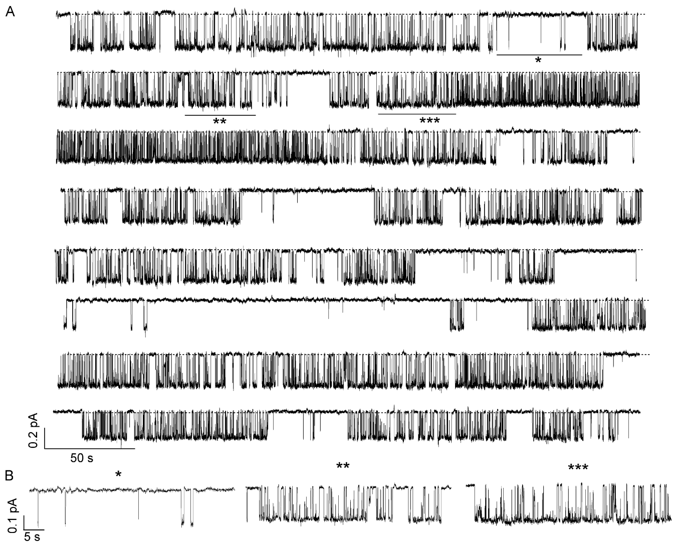
FIGURE 5. Single-channel recording of \Delta R/E1371S -CFTR in the presence of 10 \mu M ATP. (A) A continuous 45-min single-channel trace in the presence of 10 \mu M ATP. Note that the channel remains closed for long periods, and presents opening bursts of different lengths. (B) Expanded traces of selected parts of the trace in A. Note the presence of very brief openings (*), and intermediate locked-open events (**), and rarely occurring long locked-open events (***)
