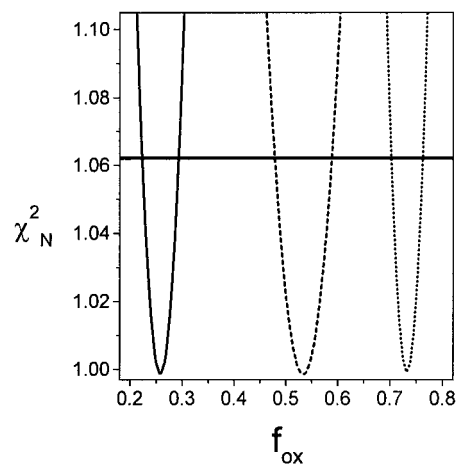
FIGURE 11 Normalized error surfaces for f_{\text{ox}} recovered for oxidatively modified CaM. Representative set of normalized chi-squared ( \chi_N^2 ) error surfaces obtained for the calculated fraction ( f_{\text{ox}} ) of CaM whose structure around PMal at Cys 26 is altered upon methionine oxidation subsequent to exposure to \text{H}_2\text{O}_2 for 1 h (solid line), 2 h (dashed line), and 4 h (dotted line), is depicted for the frequency domain data set shown in Fig. 10 and is obtained by fixing the individual values of f_{\text{ox}} associated with a particular data set, and then minimizing the simultaneous fit associated with all four data sets to a two-state model ( \text{N} \longleftrightarrow \text{O} ), where \chi_N^2 = \chi_{\text{R}}^2 / \chi_{\text{R}}^2(\text{minimum}) . This analysis quantitatively accounts for the cross-correlation between the calculated f_{\text{ox}} and the recovered lifetime parameters (i.e., \alpha_i 's and \tau_i 's), as described previously (Beechem et al., 1991). The thick horizontal line at \chi_N^2 = 1.062 corresponds to the F -statistic, which represents one-standard deviation relative to the best fit to the data. For comparison purposes, the actual distribution of oxidatively modified CaM species is documented in Table 2.
