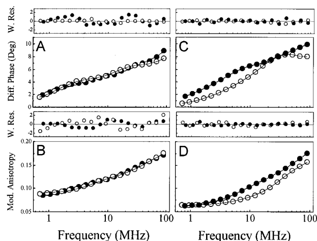
FIGURE 14 Frequency domain fluorescence anisotropy data for native and oxidatively modified CaM. Differential phase angle (A, C) and modulated anisotropy (B, D) of native CaM (○) or subsequent to exposure to H 2 O 2 for 10 h (i.e., CaM ox ; ●) for calcium-saturated (A, B) and apo- (C, D) CaM. Lines represent the best fit to the data. Weighted residuals correspond to the experimental data minus the calculated value for the two-exponential experimental fit normalized by the assumed standard errors for the measurements, which were respectively assumed to be 0.2° and 0.005 for the differential phase and modulated anisotropy. Experimental conditions involved 1.2 \mu\text{M} PMal-CaM in buffer A in the presence of either 0.1 mM CaCl 2 (A, B) or 0.1 mM EGTA (C, D). The sample temperature was 25°C.
