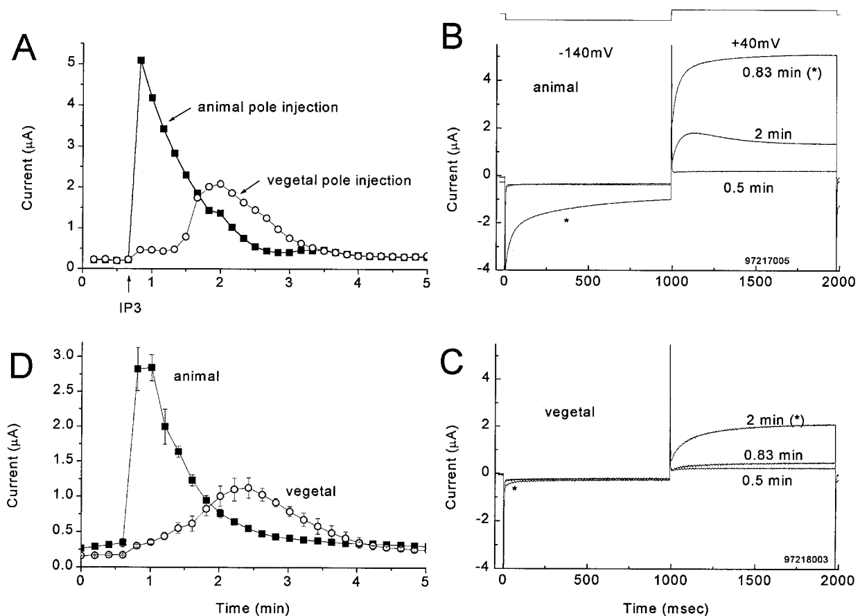
FIGURE 2 Time course of development of I Cl-1 after injection of IP 3 into animal or vegetal hemispheres. Oocytes were bathed in normal [Cl] and voltage clamped with a 1-s pulse to -140 mV, followed by a 1-s pulse to +40 mV from a holding potential of -35 mV. Stimulation was applied once every 10 s. Twenty-three nanoliters 1 mM IP 3 was injected after the fourth stimulation. (A) Typical plot of the amplitude of I Cl-1 measured as the current at the end of the +40-mV pulse. ■, Animal pole IP 3 injection. ○, Vegetal pole IP 3 injection. (B) Current traces corresponding to squares in A (animal pole IP 3 injection). Times refer to the times on the x axis in A. The asterisk identifies the trace at 0.83 min. (C) Current traces corresponding to circles in A (vegetal pole IP 3 injection). The asterisk identifies the trace at 2 min. (D) Average time course of effect of IP 3 injection into 10 oocytes injected in the animal pole (■) and 10 oocytes injected in the vegetal pole (○).
