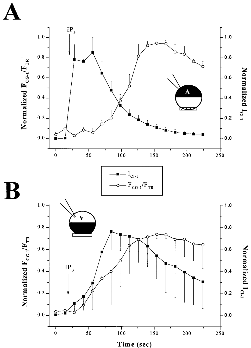
FIGURE 3 Correspondence between I_{Cl-1} and Ca signals at the animal and vegetal poles measured by confocal microscopy. Oocytes were injected with 70 kDa dextran coupled to Ca-Green-1 and Texas Red and were voltage clamped with two microelectrodes. Oocytes were voltage clamped from a holding potential of -35 mV to +40 mV for 2 s and then to -140 mV for 2 s (Hartzell, 1996). The ratio of the Ca-Green-1 (CG-1) and Texas Red (TR) fluorescence intensities was computed for the entire confocal section near the membrane ( F_{CG-1}/F_{TR} ) during the pulse to +40 mV ( \circ ). I_{Cl-1} was measured as the maximum outward current at +40 mV ( \blacksquare ). (A) IP_3 was injected into the animal hemisphere after the second pulse, as indicated by the arrow. The confocal image plane was in the vegetal hemisphere and is indicated by the hatched box. The data represent the average \pm SE of four cells. (B) IP_3 was injected into the vegetal pole after the second pulse, as indicated by the arrow. The confocal image plane was in the animal hemisphere and is indicated by the open box. The variability in the Ca fluorescence appears larger in this case because the signal was much smaller than in the opposite orientation (A), because of the pigmentation in the animal pole. I_{Cl-1} currents also appear more variable because currents obtained after IP_3 injection in the vegetal pole were smaller than those obtained after IP_3 injection in the animal pole (see Fig. 2). The data represent the average \pm SE of four cells.
