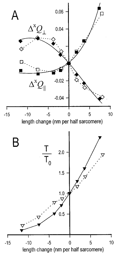
FIGURE 5 Amplitudes of {}^xQ_{\parallel} and {}^xQ_{\perp} transients (A) and tension (B), in active contraction plotted against the size of the length step. Filled symbols represent the deflections at the end of the length step (the elastic response). Open symbols represent the deflections after the quick recovery in tension (see Results). Squares and diamonds represent the deflections of {}^xQ_{\parallel} and {}^xQ_{\perp} , respectively. The smooth curve is calculated from a model presented in the Discussion. Tension ( T/T_0 ) was normalized to the isometric tension before the length step ( T_0 ). The sarcomere length change was measured at the same time point as the Q and the tension measurements. Data are from the same fiber as in Fig. 4.
