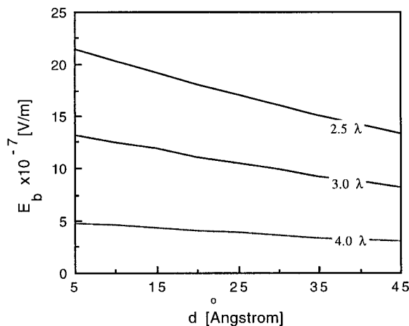
FIGURE 2 Electrostatic field strength within the granule lipid bilayer as a function of the distance, d , from the cytoplasm- membrane interface, calculated for intermembrane separations, z , of 2.5, 3.0, and 4.0 Debye lengths. R = 10 nm.
