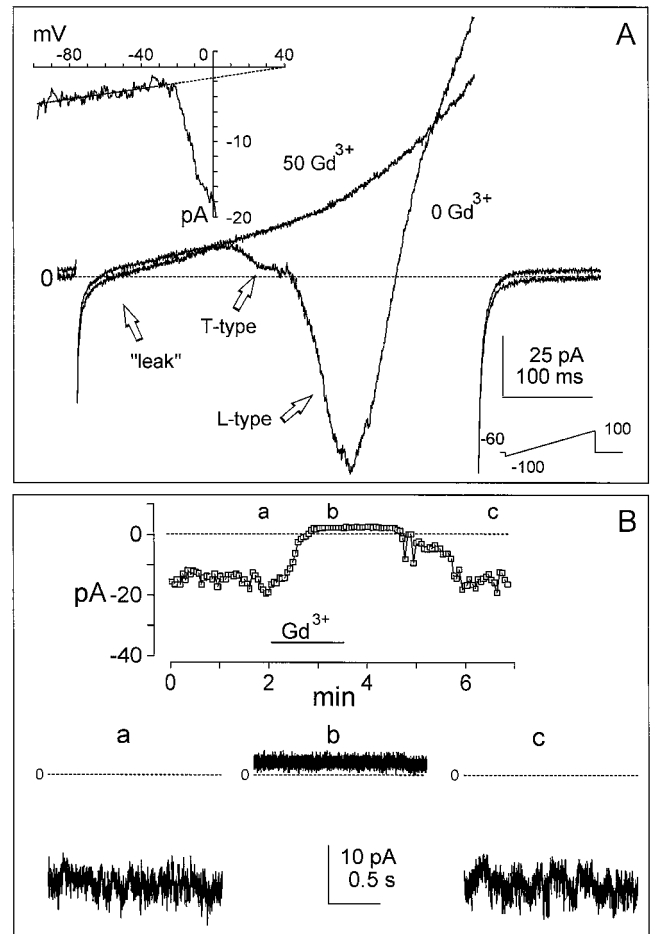
FIGURE 12 Whole-cell currents in isotonic Ba 2+ . (A) Currents during voltage ramps from -100 mV to +100 mV before (0 Gd 3+ ) and after exposure to 50 mM Gd 3+ (50 Gd 3+ ) in a perforated patch-clamp experiment. In each condition four currents were averaged. Inset : Difference current ± Gd 3+ , from -100 to 0 mV. The straight line was fitted from -90 to -30 mV. Cell a7701, whole-cell capacitance = 27.4 pF. (B) Currents at -60 mV with isotonic Ba 2+ in the classical whole-cell configuration. Each point represents the average of 16,384 samples recorded at 5000 Hz. Sample records taken at the indicated times are shown below. Cell c7908, whole-cell capacitance = 16 pF.
