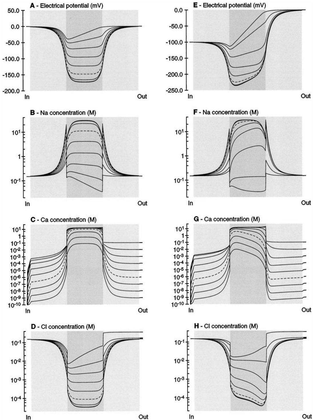
FIGURE 4 Profiles of electric potential and Na, Ca, and Cl ion concentrations as a function of bulk extracellular [Ca]. These profiles correspond to the I/V relationships plotted in Fig. 3. Two transmembrane potentials are represented: 0 mV (A–D) and -100 mV (E–H). The abscissa is nonlinear; the bulk section (white background) and atrial sections (light gray) are compressed 100- or 2-fold compared to the pore proper (darker gray). The actual dimensions are given in Fig. 1. The solutions contained 150 mM NaCl (pH 9); \text{CaCl}_2 was added to the extracellular solution in 10-fold increments from 10^{-9} to 10^{-1} M (the curves corresponding to 1 \mu\text{M} Ca are shown as dashed lines).
