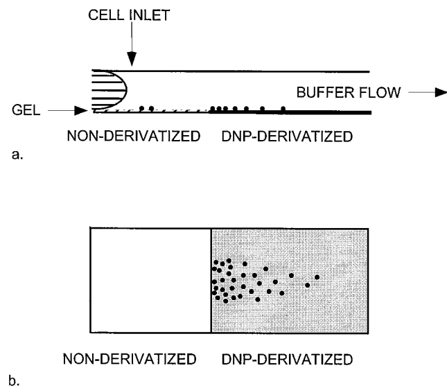
FIGURE 4 Side (a) and top (b) views of parallel-plate flow chamber. Nominal flow channel dimensions are 7 \times 2 \times 0.04 cm (L \times W \times H). IgE-sensitized cells are injected via cell inlet and allowed to settle through stationary buffer on a nonderivatized (DNP-free) portion of the gel substrate. Buffer flow is initiated, and cells are convected over and in contact with the DNP-derivatized portion of the gel substrate. Cell translational velocity is measured during perfusion via video microscopy. The population extent of adhesion and the cell spatial pattern are measured postflow via automated scanning video microscopy.
