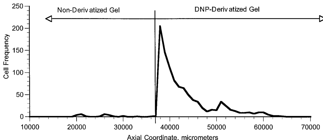
FIGURE 6 Cell binding as a function of axial position is obtained by integrating the cell density profile shown in Fig. 5 over the width of the chamber. The exponential decrease in cell frequency is fit to Eq. 2 for calculation of k_{ad} , as indicated in Materials and Methods.
