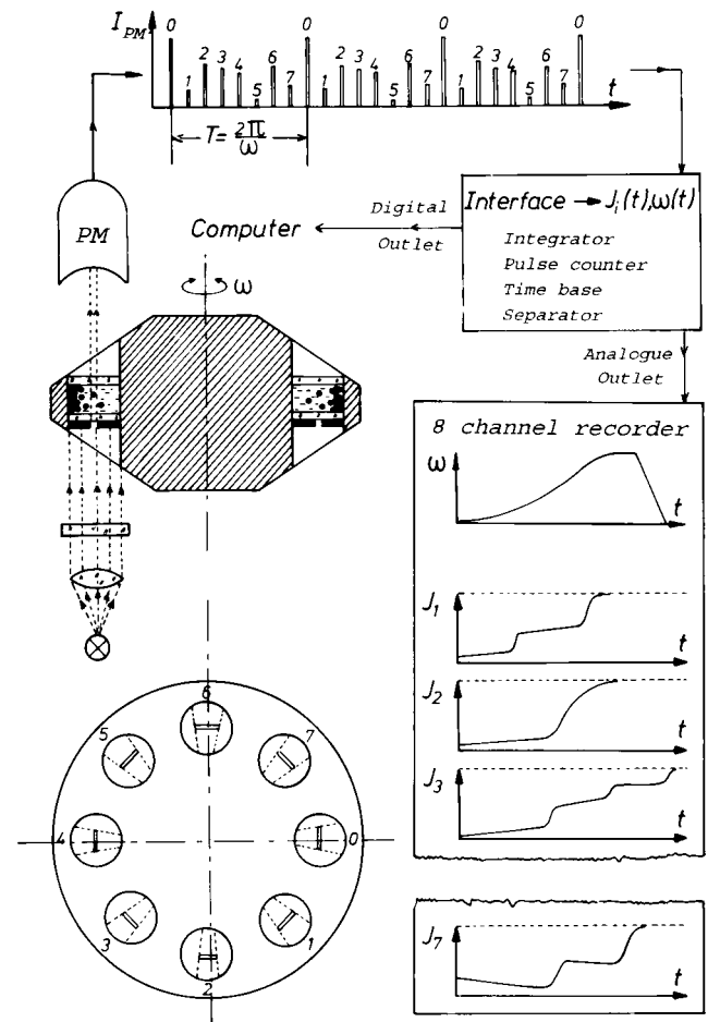
FIGURE 3 Schematic diagram of the PSD-determination method as implemented in the author's laboratory. Signal processing is synchronized to the spinning rotor by the tallest intensity spike, created by filling one cell with water. This intensity also serves as the reference intensity ( I_0 ) used in calculating the turbidity.
