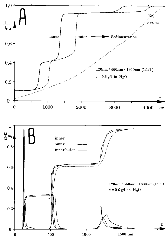
FIGURE 11 (A) Two I(t) curves of a mixture of three monodisperse polystyrene calibration latices measured simultaneously with the two-laser-beam setup in an UC. (B) Three PSD curves of a mixture of three monodisperse polystyrene calibration latices, calculated from the two I(t) curves in A and the difference curve I(t)_{inner} - I(t)_{outer} . Both the integral and differentiated curves are shown.
