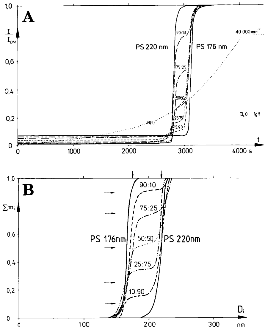
FIGURE 7 (A) The resolving power of ultracentrifuge PSD analysis. I(t) curves for seven mixtures of two monodispersed polystyrene calibration latices (176 nm + 220 nm) are shown. —, intensity curves obtained for the pure components; - - -, results from the different mixtures; \cdots , time dependence of the rotor speed. (B) When the data shown in Fig. 11 are transformed according to the Stokes-Mie theory, the resultant PSD curves are produced. —, the two pure components; - - -, data for the mixtures. The vertical arrows show the radius for each of the components. The horizontal arrows show the known mixing ratios.
