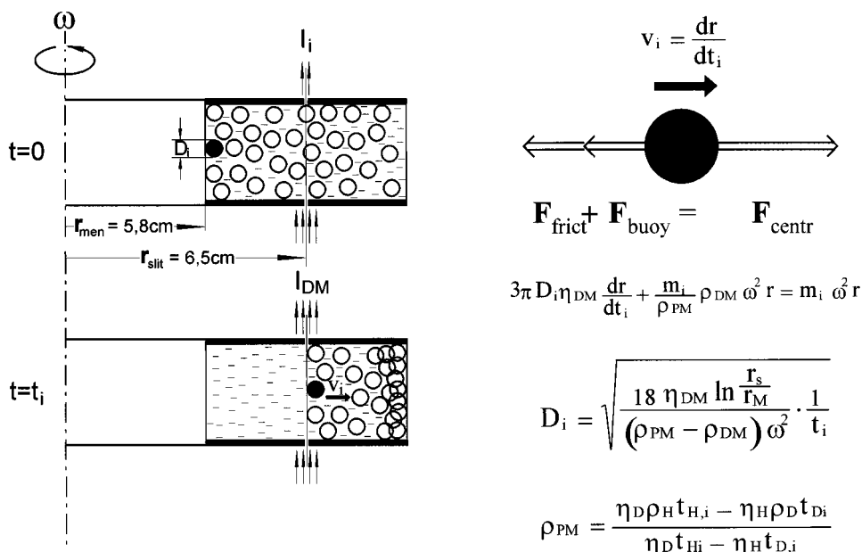
FIGURE 4 Determination of spherical particle diameter D and density \rho_{PM} using Stokes' equation. The balance of forces K_i results in the differential equation shown, which can be solved for the particle diameter if the solvent viscosity \eta_m , density \rho_{DM} , and particle density \rho_{PM} are known. The latter can be determined from the difference in sedimentation time in H_2O and D_2O dispersants.
