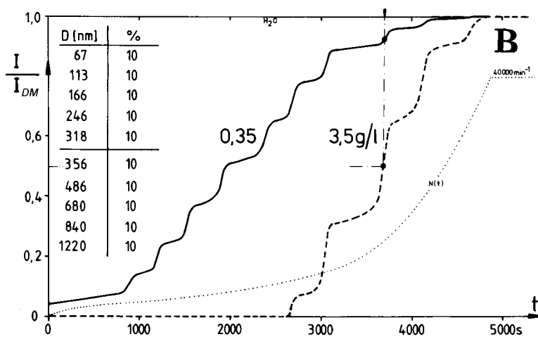
FIGURE 8 (A) PSD analysis for 10 different polystyrene latices, each with a narrow size distribution. An equal weight percent mixture of these 10 samples was made to demonstrate the ability of the coupling-PSD technique to resolve broadly distributed mixtures. (B) The intensity profiles for a low concentration (0.35 mg/ml, —) and high concentration (3.5 mg/ml, - - -) analysis of a mixture (equal weight percent) of the 10 latices shown in A. ···, time dependence of the rotor speed. The arrow and vertical dashed line shows the time point where the two intensity curves were later spliced together. (C) Resultant PSD curve for the spliced data shown in B. The coupling point where the data from different loading concentrations was spliced together is marked by the vertical dashed line. The integral distribution (heavy line) and differential distribution (light line) are shown.
