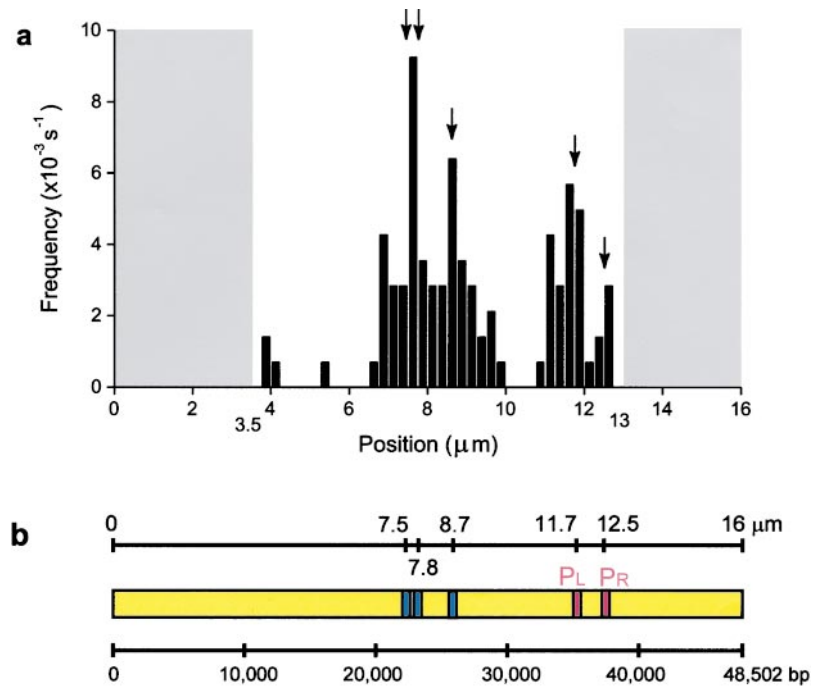
FIGURE 4 Localization of RNA polymerase molecules bound to \lambda -phage DNA for more than 1.5 s (a) Histogram of the number of RNA polymerase molecules bound to DNA. Arrows indicate the positions of the promoters and pseudopromoters, as shown in b. Bin width, 0.25 \mu\text{m} . (b) Positions of the promoters ( P_L , P_R ) and sequences common to promoters (pseudopromoters, blue-black strips). Sequences common to promoters were searched according to the method of McClure (1985).
