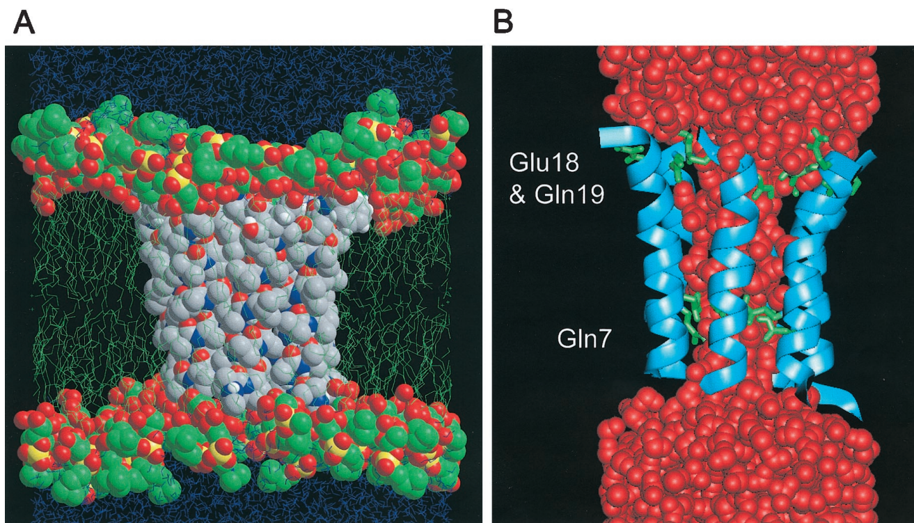
FIGURE 1 (A) Starting configuration of the simulation system for an Alm hexameric helix bundle ( cpk colors ) inserted in a POPC bilayer ( green ) with water ( cyan ) on either side. The carbonyl oxygen atoms of the acyl chains of the lipid molecules and the Alm molecule are shown in space-filling format. (B) Snapshot of the Alm N6H simulation showing the helix bundle ( blue, in ribbon format ), the rings of Gln 7 , Glu 18 , and Gln 19 side chains ( green, in stick format ), and water molecules ( red, in space-filling format ) within the pore and extending to either side of the mouths of the pore.
