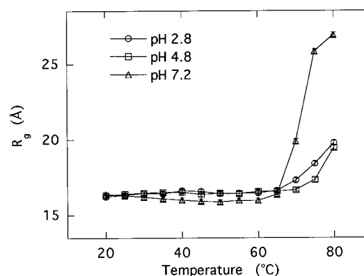
FIGURE 5 Temperature dependence of the radius of gyration R_g of the HEWL solutions (5% w/v) at different pH values. R_g values were estimated from the distance distribution functions by using Eq. 4 to the p(r) functions in Fig. 4.
