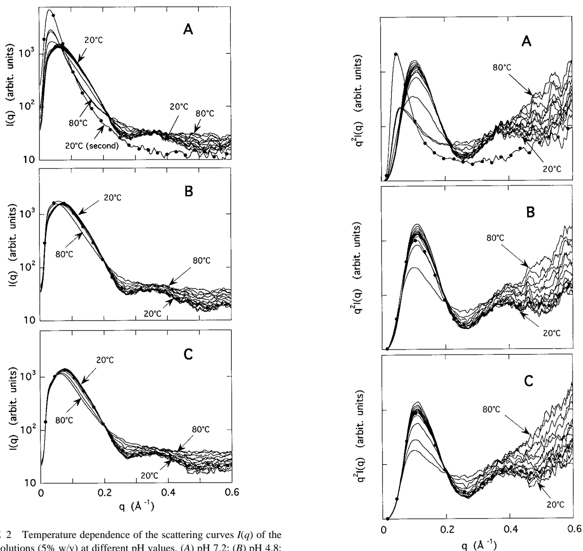
FIGURE 3 Temperature dependence of the Kratky plots ( q^2 \times I(q) vs. q plots) of the scattering curves in Fig. 2. A, B, and C and the solid lines with \bullet are as in Fig. 2.
