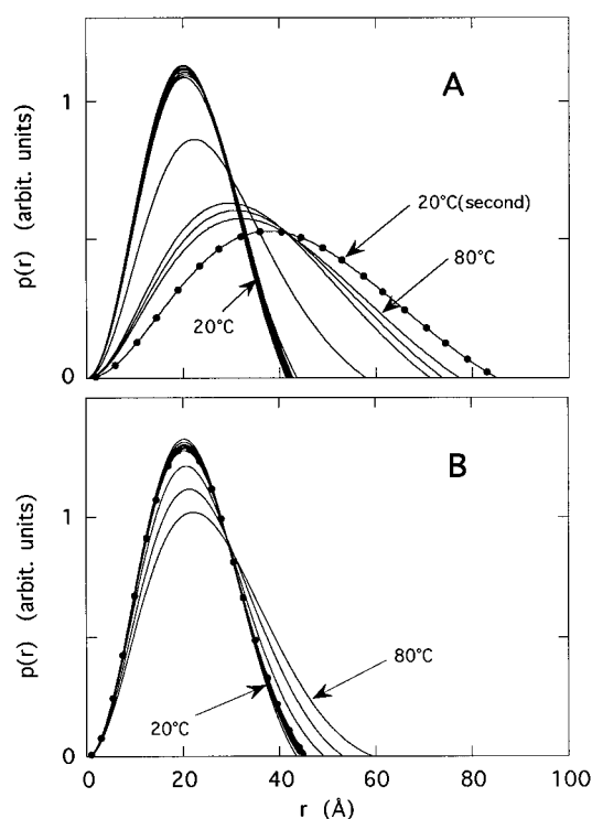
FIGURE 4 Distance distribution functions p(r) calculated by the Fourier inversion of the scattering curves in Fig. 2. (A) pH 7.2; (B) pH 2.8. The solid lines with \bullet are as in Fig. 2.
