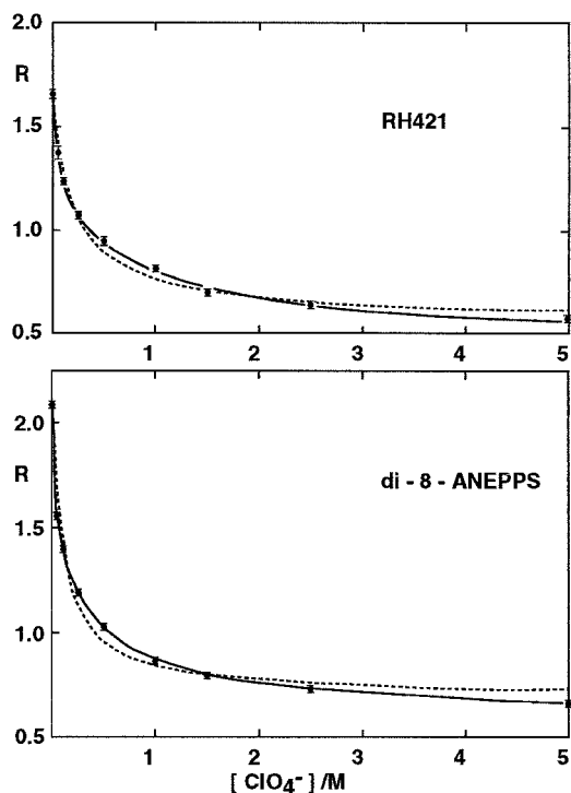
FIGURE 4 Fluorescence intensity ratios, R , of 4.1 \mu\text{M} RH421 ( top ) and 5.0 \mu\text{M} di-8-ANEPPS ( bottom ) in the presence of DMPC vesicles (3 mM lipid) as a function of the \text{NaClO}_4 concentration included in the buffer medium. The excitation and emission wavelengths were as given in Fig. 3. T = 30^\circ\text{C} , bandwidths = 5 nm. The dotted lines represent fits of the data to a binding model according to Eq. 4, excluding any electrostatic effects. The solid lines represent fits of the data to an extended binding model, described by the combination of Eqs. 4 and 5, including electrostatic repulsion effects from bound perchlorate ions.
