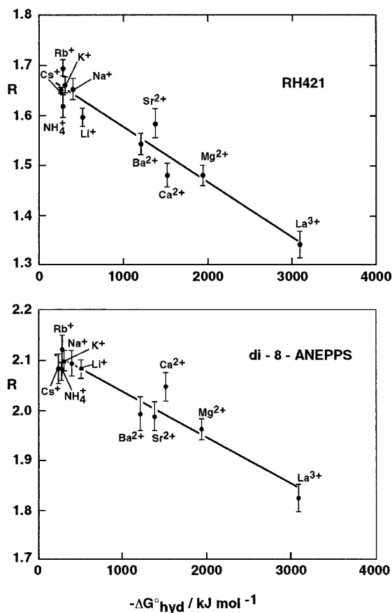
FIGURE 5 Fluorescence intensity ratios, R , of 4.1 \mu\text{M} RH421 ( top ) and 5.0 \mu\text{M} di-8-ANEPPS ( bottom ) in the presence of DMPC unilamellar vesicles (3 mM lipid) and 0.5 M of a range of chloride salts as a function of the Gibbs free energy of hydration of the relevant cations, \Delta G_{\text{hyd}}^0 . The solid line represents a fit of the data to a straight line according to Eq. 6. The values of \Delta G_{\text{hyd}}^0 are theoretical values calculated by Marcus (1991). The excitation and emission wavelengths were as given in Fig. 3. T = 30^\circ\text{C} , bandwidths = 5 nm.
