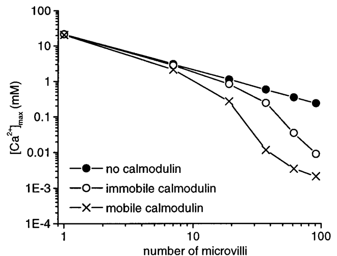
FIGURE 9 Peak values of the spatial average of [Ca^{2+}]_i in the microvillus (from Fig. 8) versus the number of microvilli participating in the bump. Without calmodulin (solid circles), the peak of [Ca^{2+}]_i reduces linearly with the number of participating microvilli. The immobile calmodulin (open circles) causes an additional reduction of the peak of [Ca^{2+}]_i , compared to the situation without calmodulin, when more than 19 microvilli participate. The mobile calmodulin (crosses) already causes this additional reduction when more than 7 microvilli are considered. However, when no more than 25 microvilli are assumed to participate in the production of a bump, the peak of the spatially averaged [Ca^{2+}]_i is higher than 80 \mu M for all buffer models.
