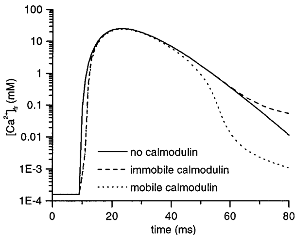
FIGURE 7 Time courses of the spatial average of [\text{Ca}^{2+}]_f in a microvillus calculated with different calcium buffer models: no calmodulin present in the microvillus ( solid line ), 0.5 mM immobile calmodulin with 4 \text{Ca}^{2+} binding sites ( dashed line ), and 0.5 mM mobile calmodulin with 4 \text{Ca}^{2+} binding sites and diffusion coefficient D_{\text{cam}} = 100 \mu\text{m}^2\text{s}^{-1} ( dotted line ). The macroscopic binding constants of the 4 binding sites of Drosophila calmodulin are taken from Maune et al. (1992). The association and dissociation reactions of \text{Ca}^{2+} with the calmodulin are assumed to be in equilibrium and are described by the Adair–Klotz-equation (Eq. 10; see text). The calculations assume the permeability ratios of TRP channels (case 1, Table 2) and that a bump is produced in a single microvillus. The calmodulin influences the dynamics of [\text{Ca}^{2+}]_f , but has virtually no effect on the peak of [\text{Ca}^{2+}]_f reached during a bump.
