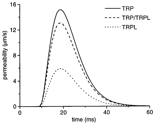
FIGURE 3 Time course of the total light-activated permeability, P_1 , during a quantum bump for three different permeability ratios (Table 2).
