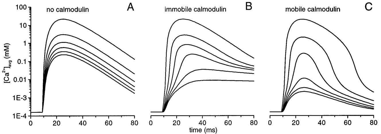
FIGURE 8 Time courses of the (spatial) average of [Ca^{2+}]_i in a microvillus assuming that more than one microvillus participate in a bump. The lines from top to bottom of each panel correspond to 1, 7, 19, 37, 61, and 91 microvilli participating in a bump, respectively. In the calculations, the permeability ratios of TRP channels are assumed (case 1, Table 2). (A) No calmodulin; (B) 0.5 mM immobile calmodulin with 4 Ca^{2+} binding sites; (C) 0.5 mM mobile calmodulin with 4 Ca^{2+} binding sites and a diffusion coefficient D_{cam} = 100 \mu m^2 s^{-1} is assumed. In all cases, the Ca^{2+} binding to phospholipids is included in the model (see text for details on Ca^{2+} buffers).
