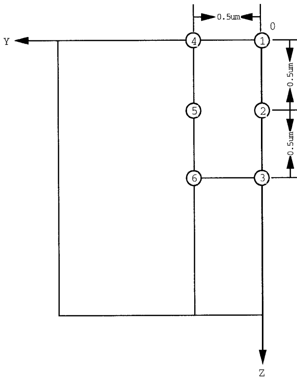
FIGURE 3 Positions of the six simulated scan lines. Line 1 , corresponds to the confocal line scan through the location of the \text{Ca}^{2+} release site. Line 2 and line 3 are two lines with the same optical axis of line 1 , but defocused by 0.5 \mu\text{m} and 1.0 \mu\text{m} from the release site, respectively. Lines 4 , 5 , and 6 are along the same optical axis, but 0.5 \mu\text{m} away from the optical axis of line 1 . Line 5 and line 2 are on the same focal plane, and so are the line 6 and line 3 .
