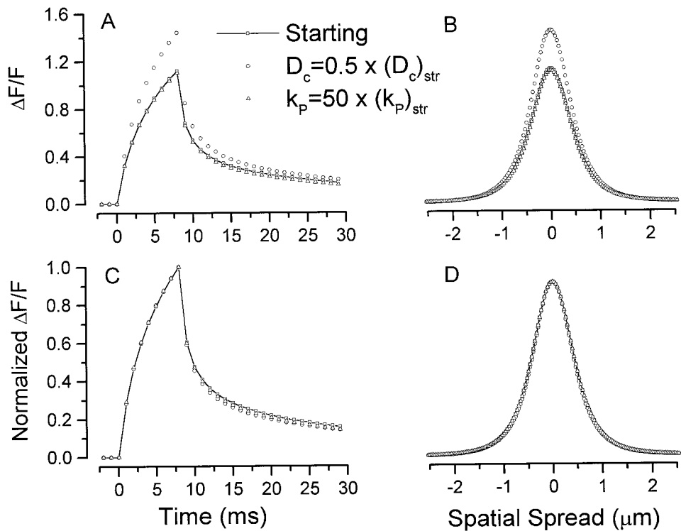
FIGURE 6 Comparisons of the results from a simulation with starting parameters ( \square ) and those from the simulations with reduced Ca 2+ diffusion coefficient ( \circ , D_c was changed from 7.0 \times 10^{-1} to 3.5 \times 10^{-1} \mu\text{m}^2\text{ms}^{-1} ) and increased rate constant for translocation of Ca 2+ ions by the SR Ca 2+ pump ( \triangle , rate constant for translocation of Ca 2+ was increased from 4.0 \times 10^{-4} to 2.0 \times 10^{-2} \text{ms}^{-1} ). (A) Comparison of time courses. (B) Comparison of spatial spreads. (C) and (D) are (A) and (B) normalized with respect to the corresponding peak of each line.
