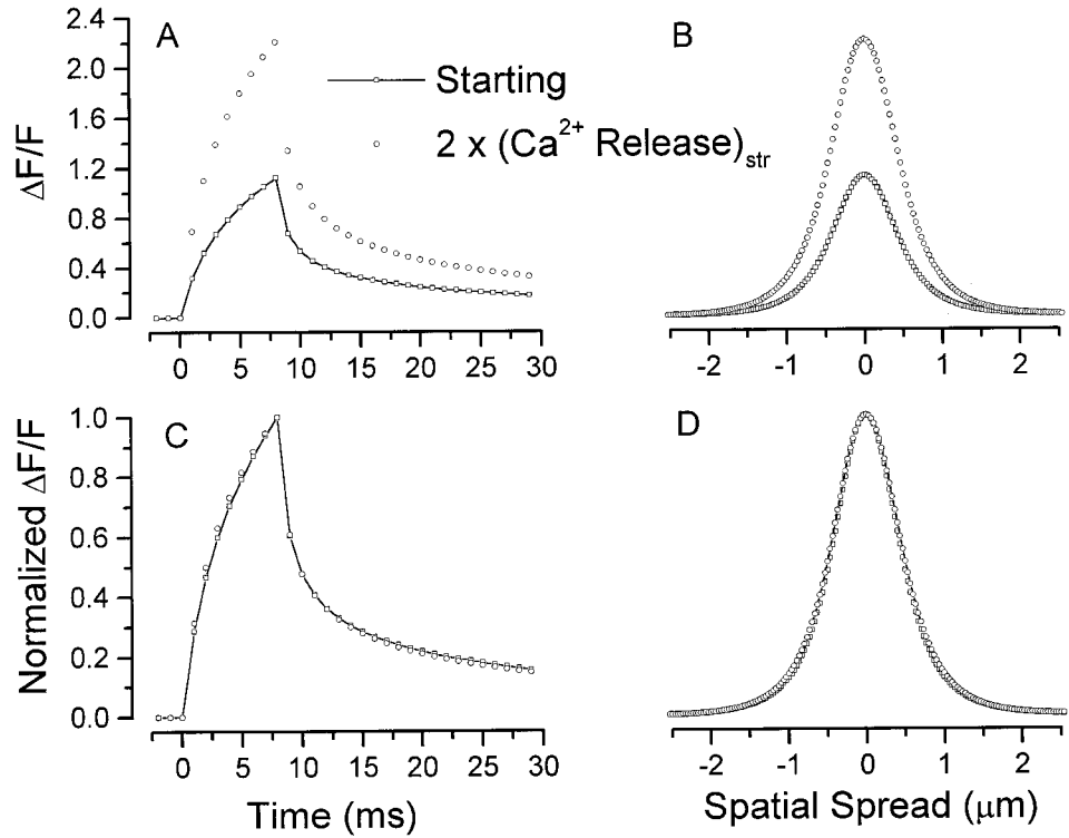
FIGURE 5 Comparisons of the results from a simulation with starting Ca 2+ release current ( \square , 1.4 pA) and those from a simulation with doubled Ca 2+ release current ( \circ , 2.8 pA). The current duration was 8 ms in both cases. (A) Comparison of time courses. (B) Comparison of spatial spreads. (C) and (D) are (A) and (B) normalized with respect to the corresponding peak of each line.
