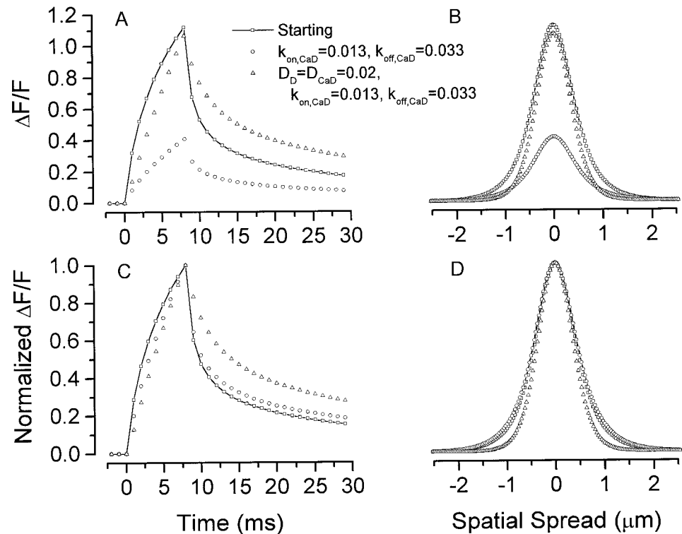
FIGURE 8 Comparison of the results under different dye kinetic properties and diffusion coefficients. \square , D_D = D_{CaD} = 9.0 \times 10^{-2} \mu\text{m}^2\text{ms}^{-1} , k_{on,CaD} = 2.36 \times 10^{-1} \mu\text{M}^{-1}\text{ms}^{-1} , k_{off,CaD} = 1.75 \times 10^{-1} \text{ms}^{-1} . \circ , D_D = D_{CaD} = 9.0 \times 10^{-2} \mu\text{m}^2\text{ms}^{-1} , k_{on,CaD} = 1.3 \times 10^{-2} \mu\text{M}^{-1}\text{ms}^{-1} , k_{off,CaD} = 3.3 \times 10^{-2} \text{ms}^{-1} . \triangle , D_D = D_{CaD} = 2.0 \times 10^{-2} \mu\text{m}^2\text{ms}^{-1} , k_{on,CaD} = 1.3 \times 10^{-2} \mu\text{M}^{-1}\text{ms}^{-1} , k_{off,CaD} = 3.3 \times 10^{-2} \text{ms}^{-1} . (A) Comparison of time courses. (B) Comparison of spatial spreads. (C) and (D) are (A) and (B) normalized with respect to the corresponding peak of each line.
