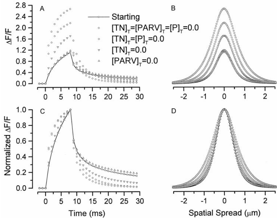
FIGURE 9 Comparisons of the results from a simulation with all starting binding sites ( \square , [\text{TN}]_{\text{T}} = 240.0 \mu\text{M} , [\text{PARV}]_{\text{T}} = 1000.0 \mu\text{M} , [\text{P}]_{\text{T}} = 200.0 \mu\text{M} , [\text{D}]_{\text{T}} = 50.0 \mu\text{M} ) and those from simulations with the elimination of different binding sites except \text{Ca}^{2+} indicator D ( \circ , [\text{TN}]_{\text{T}} = [\text{PARV}]_{\text{T}} = [\text{P}]_{\text{T}} = 0.0 , [\text{D}]_{\text{T}} = 50.0 \mu\text{M} ; \diamond , [\text{TN}]_{\text{T}} = [\text{P}]_{\text{T}} = 0.0 , [\text{PARV}]_{\text{T}} = 1000.0 \mu\text{M} , [\text{D}]_{\text{T}} = 50.0 \mu\text{M} ; \nabla , [\text{TN}]_{\text{T}} = 0.0 , [\text{PARV}]_{\text{T}} = 1000.0 \mu\text{M} , [\text{P}]_{\text{T}} = 200.0 \mu\text{M} , [\text{D}]_{\text{T}} = 50.0 \mu\text{M} ; \triangle , [\text{PARV}]_{\text{T}} = 0.0 , [\text{TN}]_{\text{T}} = 240.0 \mu\text{M} , [\text{P}]_{\text{T}} = 200.0 \mu\text{M} , [\text{D}]_{\text{T}} = 50.0 \mu\text{M} ). (A) Comparison of time courses. (B) Comparison of spatial spreads. (C) and (D) are (A) and (B) normalized with respect to the corresponding peak of each line.
