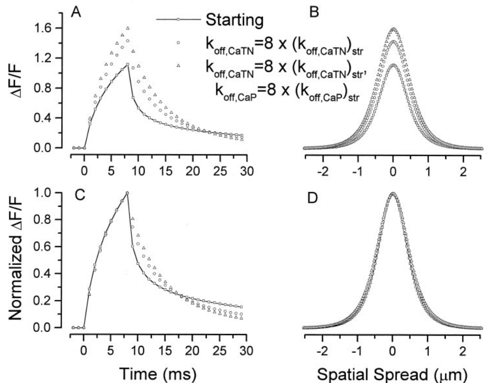
FIGURE 10 Comparisons of the results from a simulation with all starting binding properties ( \square ) and those from simulations with increased off-rate constants for the rapidly equilibrating binding sites intrinsic to the muscle fibers ( \circ , k_{\text{off,CaTN}} was increased from 1.2 \times 10^{-1} to 9.6 \times 10^{-1} \text{ms}^{-1} ; \triangle , k_{\text{off,CaTN}} was increased from 1.2 \times 10^{-1} to 9.6 \times 10^{-1} \text{ms}^{-1} , k_{\text{off,CaP}} was increased from 4.0 \times 10^{-1} to 3.2 \text{ms}^{-1} ). (A) Comparison of time courses. (B) Comparison of spatial spreads. (C) and (D) are (A) and (B) normalized with respect to the corresponding peak of each line.
