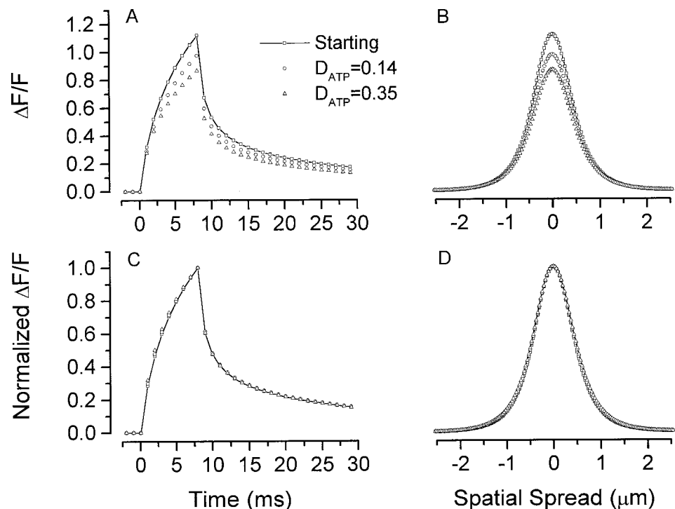
FIGURE 11 Comparisons of the results from the starting simulation, which does not include the diffusion of ATP, CaATP, and MgATP ( \square ), and those from simulations with the diffusion of ATP, CaATP, and MgATP at two different diffusion coefficients ( \circ , D_{\text{ATP}} = D_{\text{CaATP}} = D_{\text{MgATP}} = 1.4 \times 10^{-1} \mu\text{m}^2\text{ms}^{-1} ; \triangle , D_{\text{ATP}} = D_{\text{CaATP}} = D_{\text{MgATP}} = 3.5 \times 10^{-1} \mu\text{m}^2\text{ms}^{-1} ). (A) Comparison of time courses. (B) Comparison of spatial spreads. (C) and (D) are (A) and (B) normalized with respect to the corresponding peak of each line.
