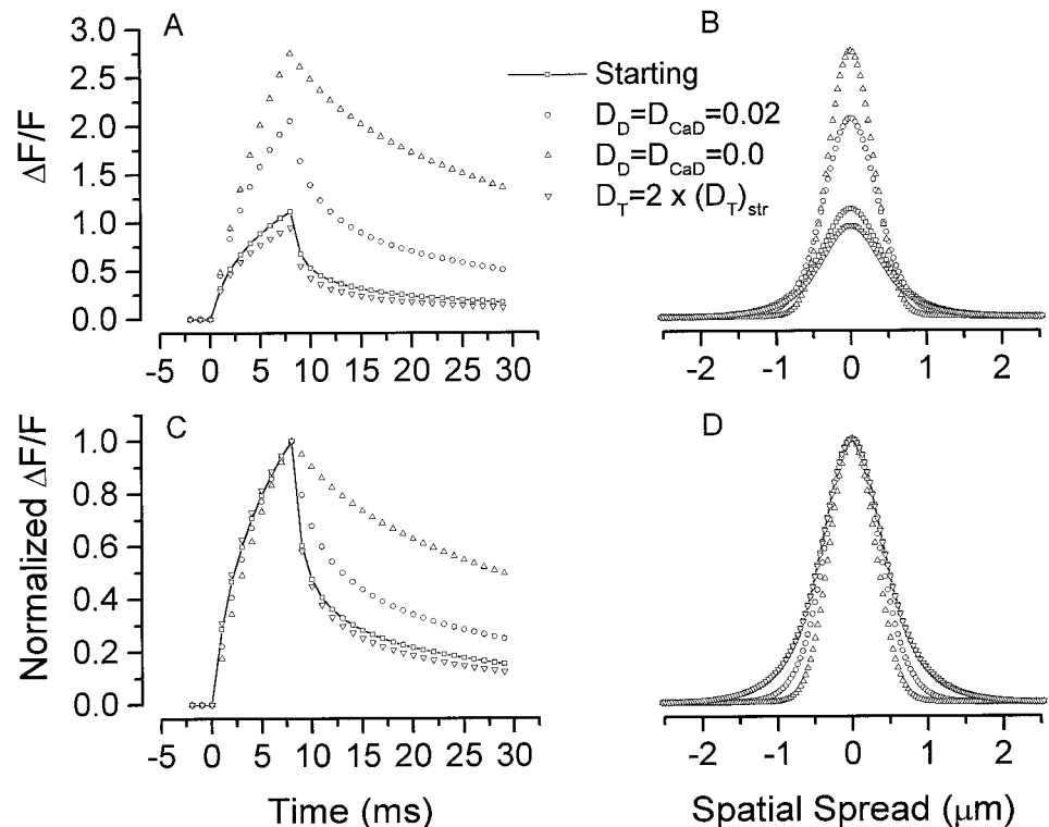
FIGURE 7 Comparisons of the results from a simulation with starting diffusion coefficients of D and CaD ( \square , D_D = D_{\text{CaD}} = 9.0 \times 10^{-2} \mu\text{m}^2\text{ms}^{-1} ) and those from the simulations with smaller ( \circ , D_D = D_{\text{CaD}} = 2.0 \times 10^{-2} \mu\text{m}^2\text{ms}^{-1} ) or zero ( \Delta , D_D = D_{\text{CaD}} = 0.0 ) diffusion coefficients of D and CaD. \nabla , simulation in which the dye concentration was increased twofold compared to the starting conditions, to 100 \mu\text{M} . (A) Comparison of time courses. (B) Comparison of spatial spreads. (C) and (D) are (A) and (B) normalized with respect to the corresponding peak of each line.
