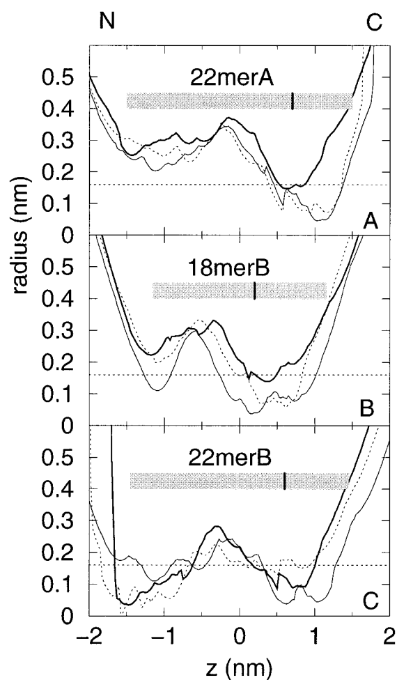
FIGURE 13 Pore radius profiles, showing important time points in the simulations. (A) 22merA with its N-terminus open at t = 0 ps (solid line), at t = 400 ps (dotted line) where its C-terminus is opening, and at t = 2 ns (thicker line). (B) 18merB at t = 0 ps (solid line), t = 50 ps (dotted line), and t = 1 ns (thicker line). (C) 22merB at t = 0 ps (solid line), t = 1400 ps (dotted line), and t = 2 ns (thicker line).
