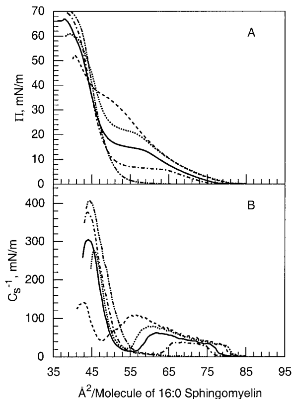
FIGURE 1 16:0 SM monolayers. Data were collected using an automated Langmuir-type film balance (see Methods). Traces at 10°C are indicated by (— · — ·); at 15°C by (— · — ·); at 20°C by (—); at 24°C by (· · ·); and at 30°C by (— — —). (A) Surface pressure versus average cross-sectional molecular area ( \pi - A ). (B) Interfacial elastic modulus of area compressibility ( C_s^{-1} ) versus average molecular area.
