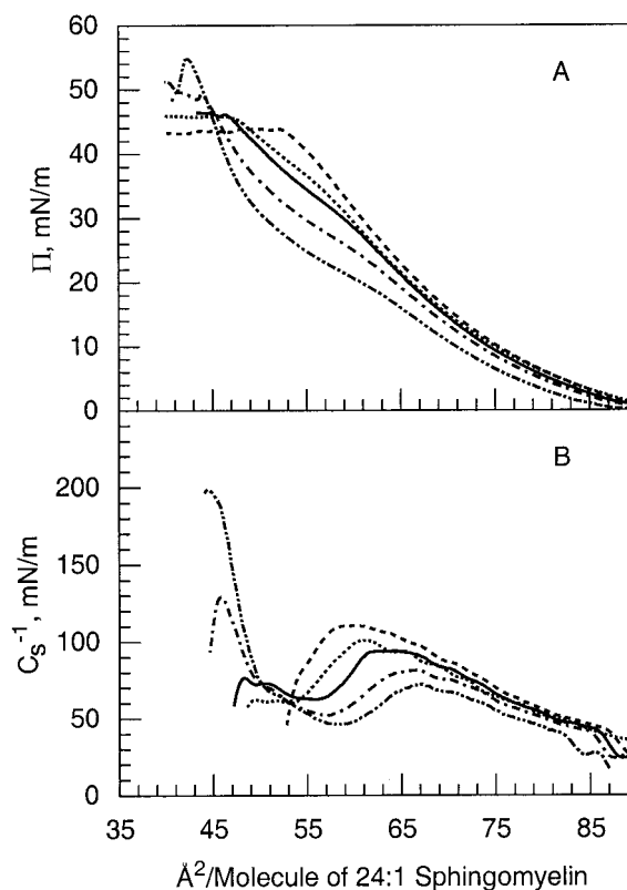
FIGURE 8 24:1 SM monolayers. (A) Surface pressure versus average cross-sectional molecular area ( \pi -A). (B) Interfacial elastic modulus of area compressibility ( C_s^{-1} ) versus average molecular area (other details same as in Fig. 1 legend).
