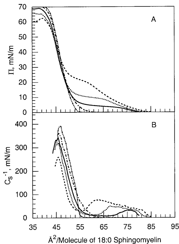
FIGURE 2 18:0 SM monolayers. (A) Surface pressure versus average cross-sectional molecular area ( \pi - A ). (B) Interfacial elastic modulus of area compressibility ( C_s^{-1} ) versus average molecular area (other details same as in Fig. 1 legend).
