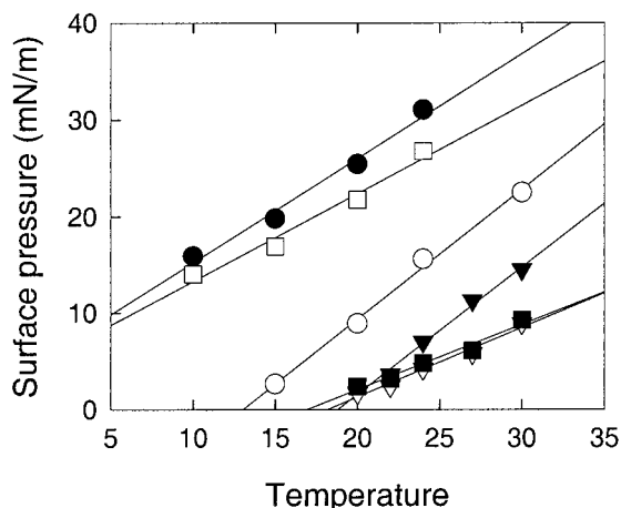
FIGURE 9 SM transition onset pressures versus temperature. Values were determined as described by Kellner et al. (1978). 14:0 SM, ●; 24:1 SM, □; 16:0 SM, ○; 18:0 SM, ▼; 24:0 SM, ▽; 26:0 SM, ■.
