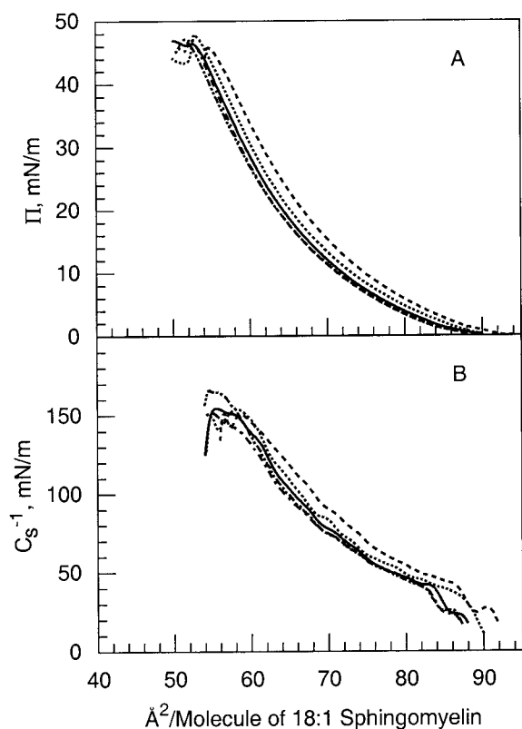
FIGURE 7 18:1 SM monolayers. (A) Surface pressure versus average cross-sectional molecular area ( \pi -A). (B) Interfacial elastic modulus of area compressibility ( C_s^{-1} ) versus average molecular area (other details same as in Fig. 1 legend).
