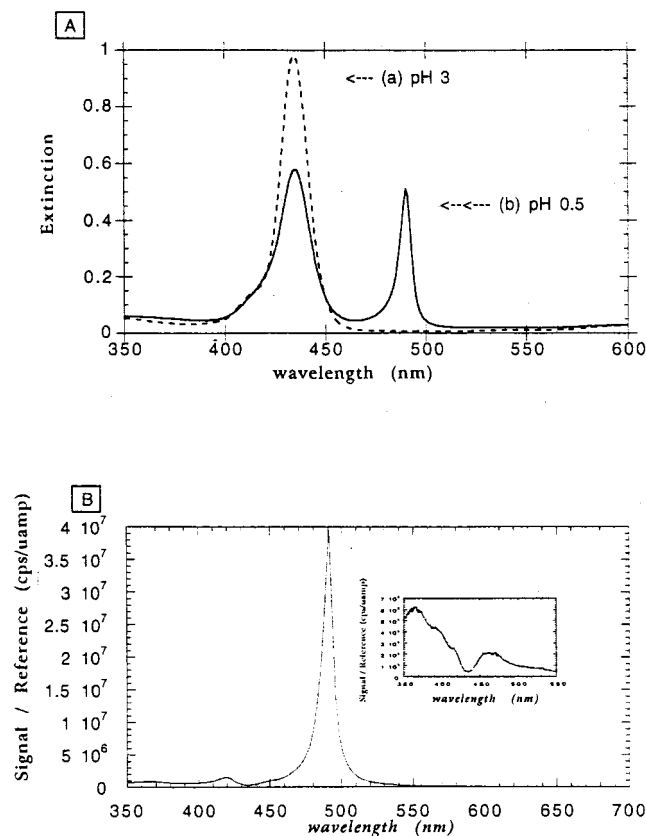
FIGURE 2 (A) Extinction spectra of H 4 TPPS 4 2- solutions at pH 3 ( curve a ) and pH 0.5 ( curve b ). The monomer Soret band of the diacid form of the porphyrin is at 435 nm; the J-aggregate produces a band of Soret intensity at 490 nm. (B) Resonance light scattering spectra of the solutions of A. The aggregate produces a markedly enhanced RLS signal at 490 nm, a small trough at 435 nm, and a smaller enhanced RLS signal near 420 nm, whereas the monomer ( inset ) shows only a trough at 435 nm.
