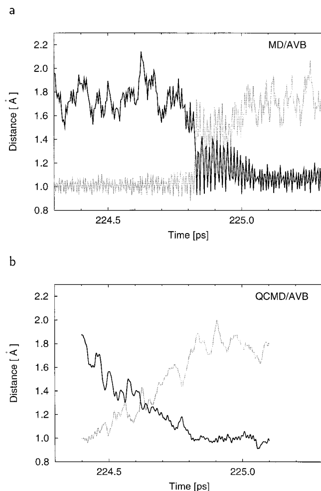
FIGURE 5 The water oxygen (OW)-hydrogen ( gray trace ) and imidazole nitrogen (ND1)-hydrogen ( black trace ) distances obtained in the MD/AVB ( a ) and QCMD/AVB ( b ) simulations.
