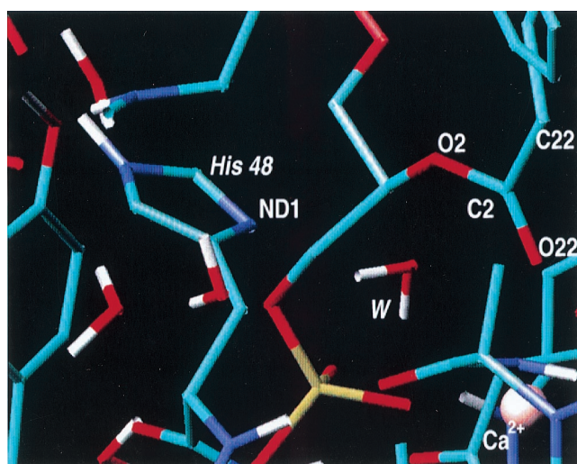
FIGURE 1 Active site of phospholipase A_2 and the substrate with the C2-O 2 ester bond to be cleaved. The water molecule (W) playing a crucial role in the catalytic process is shown in the middle.
