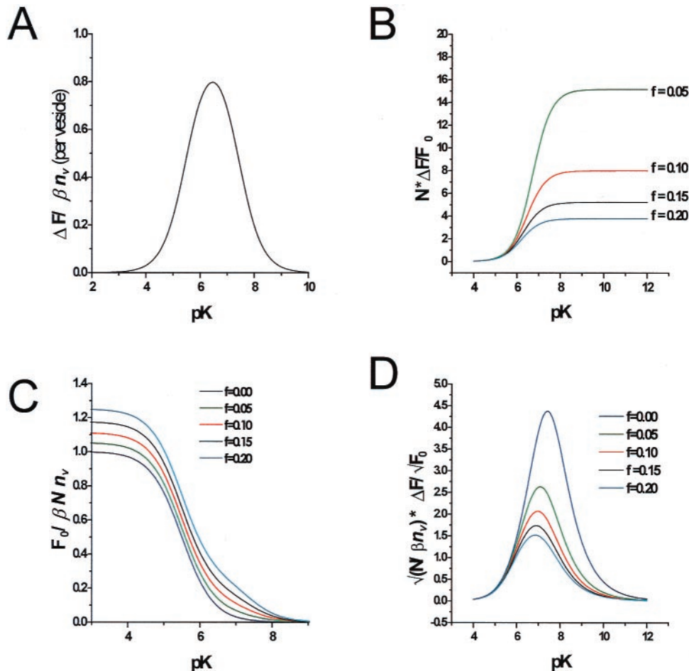
FIGURE 5 Calculation of the relationship between experimentally measured optical parameters as a function of pK and surface fraction for a fluorophore that undergoes a pH change from 5.6 to 7.4. The relationship between (A) change in fluorescence ( \Delta F ); (B) change in fluorescence relative to initial fluorescence ( \Delta F/F_0 ); (C) initial fluorescence ( F_0 ); and (D) The signal-to-noise ratio ( \Delta F/\sqrt{F_0} ) and pK of fluorophore are illustrated. The surface fractions f are denoted by the different colors in B, C, and D. The equations used to obtain the curves are Eqs. 9, 11, 10, and 12 described in the text.
