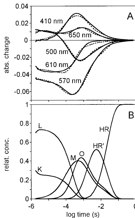
FIGURE 4 (A) the fit of the photocycle model ( broken lines ) to the absorption kinetic signals ( continuous lines ). (B) time evolution of the concentration of the intermediates. Measuring conditions were the same as in Fig. 2. The error of the fit was \pm 10\% .
