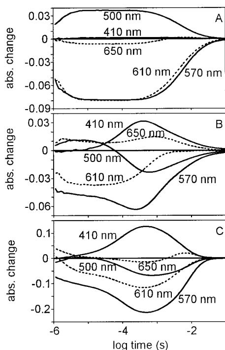
FIGURE 1 Absorption kinetic signals measured at five wavelengths on pharaonis halorhodopsin (A) and bacteriorhodopsin (C) in 1 M NaCl, 50 mM MES, pH 6, 20°C, and on pharaonis halorhodopsin (B) in 100 mM \text{NaN}_3 , 1 M \text{Na}_2\text{SO}_4 , 50 mM MES, pH 6, 20°C.
