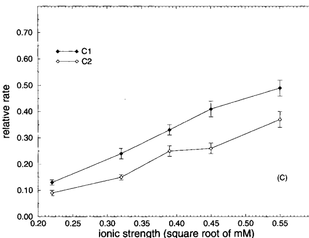
FIGURE 5 Comparison between ionic strength dependence of relative rates computed using one-distance criterion (C1) and two-distance criterion (C2), for a single mutant involving (A) residue H 35, E35Q, (B) residue H 50, E50Q, and (C) for a DMU involving both the two key residues of the binding site, E35Q + E50Q. Error bars as in caption of Fig. 4. Differences between relative rates computed with C1 and C2 that appear in the mutants arise from reduced electrostatic steering.
