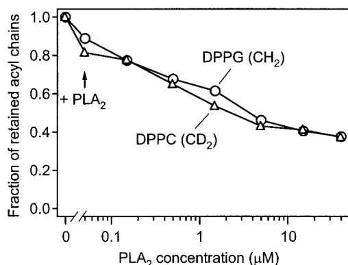
FIGURE 13 Normalized integrated intensities of methylene stretching bands of DPPG (○) and DP(d 62 )PC (△) as a function of PLA 2 concentration, calculated from the data of an experiment described in Fig. 12.
