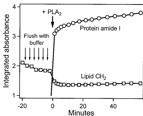
FIGURE 5 Dependence of the integrated intensities of the lipid methylene and the protein amide I bands on flushes with buffer and injection of 5 \mu\text{M} \text{PLA}_2 , as described in Fig. 4.
