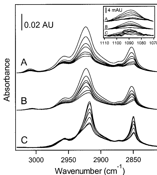
FIGURE 7 Lipid methylene (and phosphate, in the inset ) stretching bands at different concentrations of \text{PLA}_2 . The lipid composition of the asymmetric supported bilayers was as follows. (A) PLPC/(PLPC + PLPG); (B) POPC/(POPC + POPG); (C) DPPC/(DPPC + DPPG). In all three cases, the fraction of the acidic lipid in the upper leaflet is 20 mol %. The buffer contained 5 mM Hepes (pH 8.2), 100 mM NaCl, 15 mM KCl, 2 mM \text{CaCl}_2 . In each of the three families of spectra, \text{PLA}_2 concentration was increased from 0 to 50 \mu\text{M} (from top to bottom).
