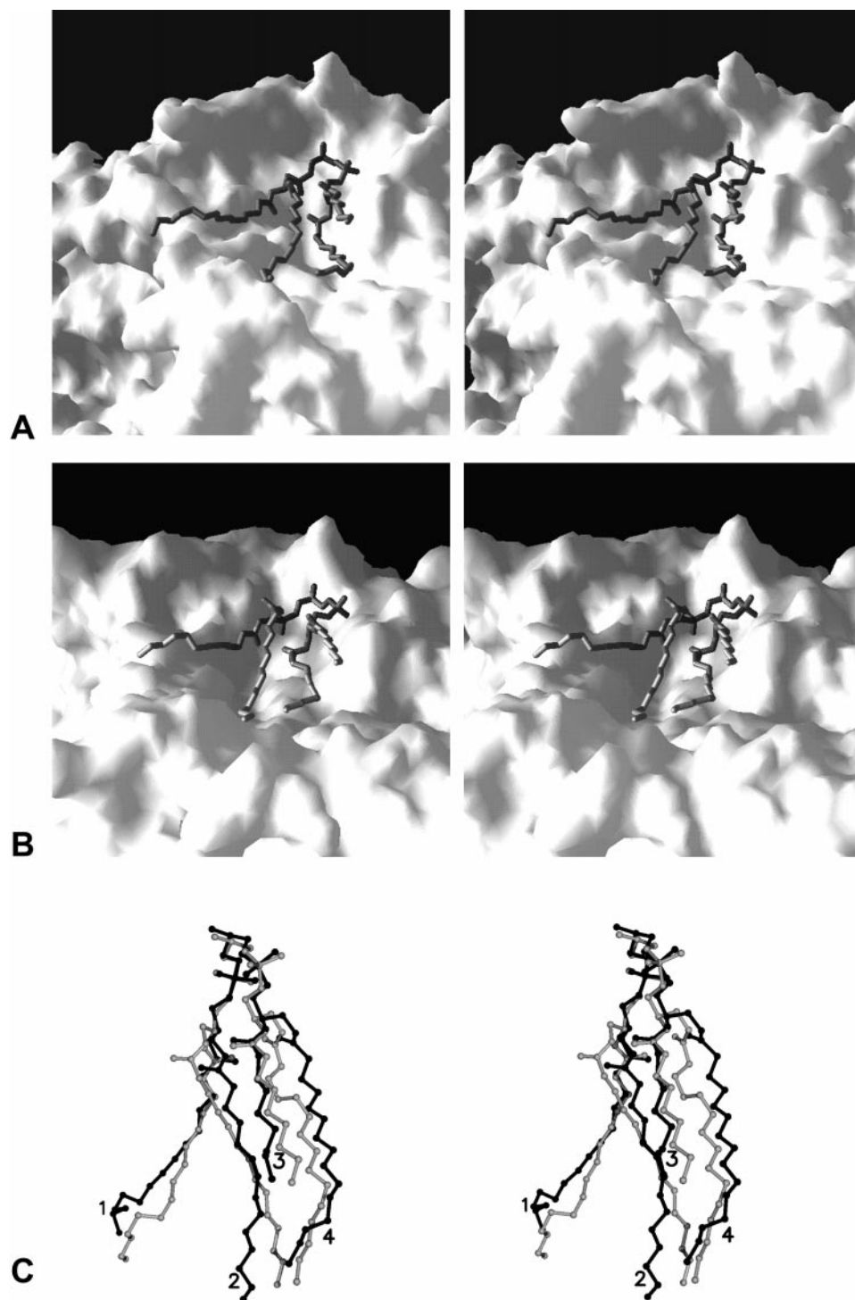
FIGURE 4 Cardiophilin in the VMOD2 model of the Rps. viridis reaction center. (A) Stereo image of a surface representation of the Rb. sphaeroides reaction center, with the crystallographically resolved cardiophilin molecule shown in stick format. The view is along the intra-membrane surface of the protein, from the periplasmic side of the membrane. (B) Stereo image showing a surface representation of the Rps. viridis reaction center, with the cardiophilin shown in stick format. (C) Stereo image of the cardiophilin molecules from the 1QOV (dark gray) and VMOD2 (light gray) models.
