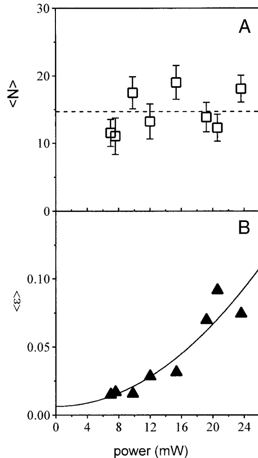
FIGURE 5 Fit of the PCHs for 1.2 \mu M OASS in 100 mM potassium phosphate, pH 7. The average number of molecules, \langle N \rangle (A), and the molecular brightness, \langle \epsilon \rangle , for a sampling time of 50 \mu s (B), are reported as a function of the excitation power at \lambda_{\text{ex}} = 775 nm. The dashed line in A indicates the average number of OASS molecules, 15 \pm 3 . The solid line in B is a square law fit of the fluorescence yield.
