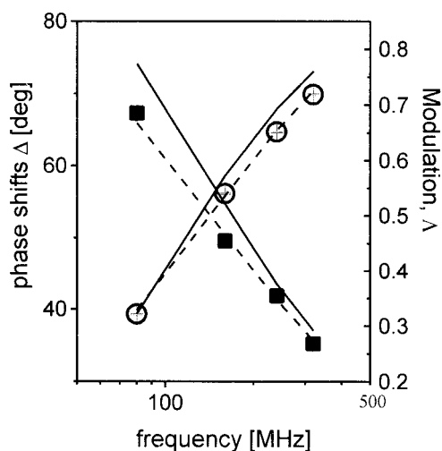
FIGURE 8 Phase shifts ( \circ , left axis) and modulations ( \blacksquare , right axis), measured at \lambda_{\text{ex}} = 775 nm for a 12 \mu\text{M} OASS solution in 100 mM potassium phosphate, pH 7. The solid and dashed lines represent a single- and a two-species fit of the data.
