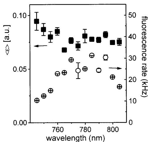
FIGURE 7 Apparent molecular brightness of OASS, \langle \epsilon \rangle ( \blacksquare , left y axis), as obtained from the best fit of PCHs for 1.2 \mu\text{M} protein in 100 mM potassium phosphate, pH 7, as a function of the excitation wavelength. The average fluorescence rate is also shown ( \circ , right y axis).
