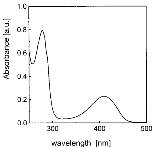
FIGURE 1 Absorbance spectrum of OASS. Enzyme protomers concentration was 29.9 \mu\text{M} in 100 mM potassium phosphate, pH 7.
