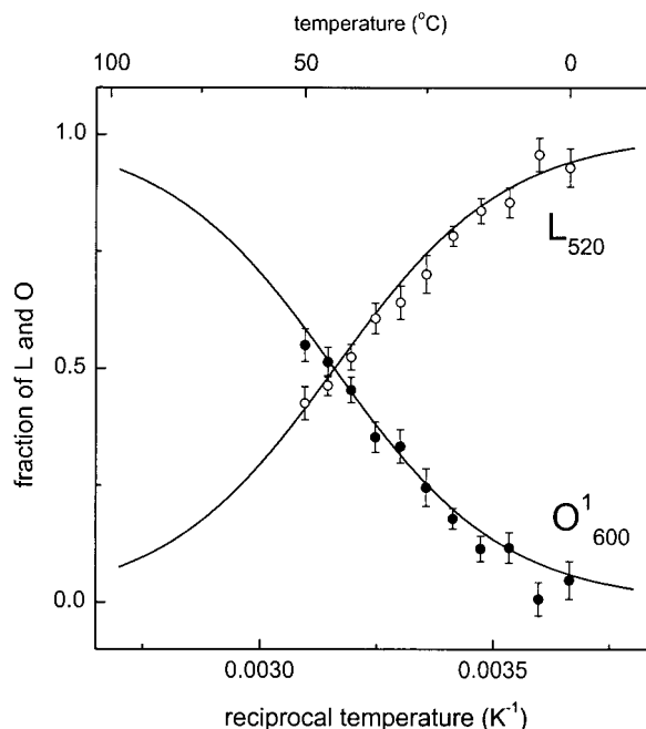
FIGURE 5 Temperature dependence of the fractions of L_{520} (○) and O_{600}^1 (●) chromophore states obtained in the P_4 kinetic state. Solid lines represent the fit of data according to the thermal equilibrium equation giving the differences of enthalpy and entropy \Delta H_{LO} = 45 \pm 5 kJ/mol and \Delta S_{LO} = 140 \pm 20 J/mol K, respectively.
