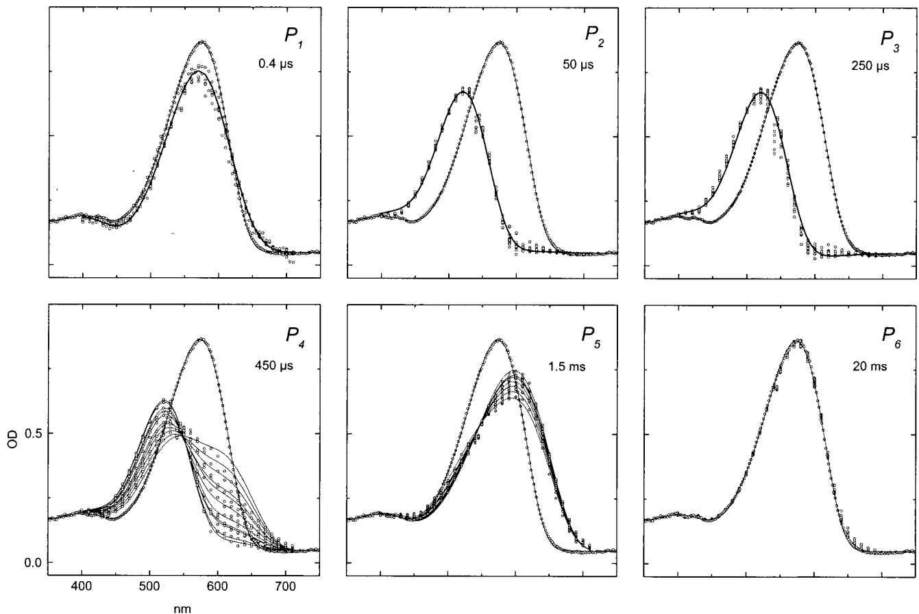
FIGURE 4 Absolute spectra of kinetic states P_1 – P_6 at temperatures between 0^\circ\text{C} and 50^\circ\text{C} (step size 5^\circ\text{C} , pH 6.0, 150 mM NaCl). Depicted half-times of transitions correspond to 20^\circ\text{C} . For reasons of comparison, the initial spectrum of pHR is also shown in each panel. The figure shows the experimental data ( \circ ) and the Gaussian fit (—) of the absorption spectrum of the initial state and those of the kinetic states P_1 – P_6 , which were fitted globally at all measured parameters (see details in the text and Table 1 for the parameters of the fitted spectra). The spectra of the first state ( P_1 ; K-like intermediate) could be reliably resolved only at T \leq 25^\circ\text{C} . The spectra were derived from the difference spectra of the kinetic states by variation of the fraction cycling. In the whole temperature range the value of the fraction cycling is 30 \pm 2\% .
