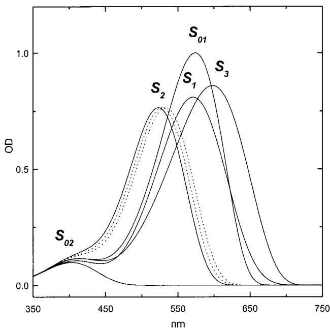
FIGURE 8 Spectra of the pHR chromophore in the initial state S_{01,02} and three major archetype spectral states of the pHR photocycle S_{1-3} deduced from the global multi-Gaussian fitting of the data in Figs. 4, 6, and 7. Dotted lines are S_2 for bromide and iodide samples. The fitted parameters are compiled in Table 1.
