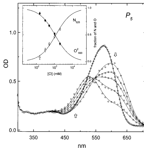
FIGURE 6 Dependence of the P_5 kinetic state on the chloride concentration. The figure shows the experimental data (○) and the Gaussian fit (—). The inset shows the fractions of N_{520} (○) and O_{600}^2 (●) chromophore states obtained in P_5 versus \log[Cl] . The hyperbolic fit of data (—) gives an equilibrium constant of K_d = 1.1 \pm 0.2 M for chloride.
