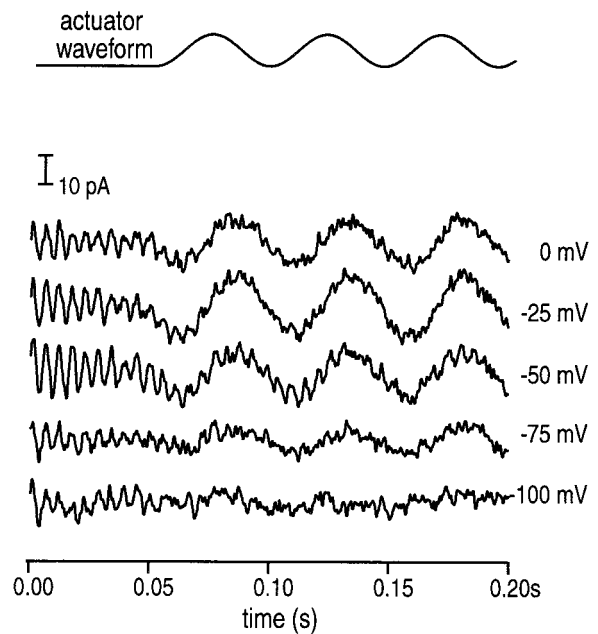
FIGURE 2 Currents by stretching outer hair cell at various holding potentials. The first 200-ms segments of the records are shown. An upward deflection of the actuator waveform stretches the cell. The peak-to-peak amplitude of probe movement is 1.24 \mu\text{m} when it is disengaged with the cell and \sim 0.35 \mu\text{m} when it is engaged. Membrane currents are monitored under whole-cell voltage clamp. The holding potentials are indicated on the right-hand side of the respective traces. Downward deflections in the current traces correspond to inward currents. On the top four current traces, currents precede probe movements by 95.4 \pm 1.4 degrees in phase (mean \pm SD). The frequency of fiber probe movement is 21 Hz. The oscillatory current of \sim 100 Hz corresponds to a resonance frequency of the probe. Probe stiffness is 8 nN/ \mu\text{m} and cell length is 59 \mu\text{m} .
