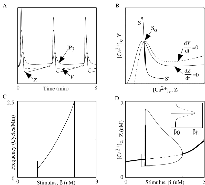
FIGURE 2 Dynamics of the voltage-dependent system. (A) Intracellular Ca^{2+} ( Z ) and membrane potential ( V ) oscillations are in phase, whereas IP_3 oscillations follow with a lag. All traces are normalized. (B) Schematic nullclines dZ/dt = 0 and dY/dt = 0 . Path of steady state as a function of F(\beta, V) given by line SS' , thick part of the line represents stable oscillations. S_0 is the instantaneous steady state of the system. The ends of the thick solid line represent the two Hopf points. (C) Frequency of oscillation plotted against stimulus \beta . (D) Bifurcation diagram for Ca^{2+} with \beta as the parameter. Oscillations arise and end through the two Hopf bifurcation points. Inset shows the bistable region, \beta_0 < \beta < \beta_h , (in box) enlarged. Stable steady states (thick solid); unstable steady states (dashed); maxima and minima of stable oscillations (solid); and unstable oscillations (dots). \beta = 0.8 \mu\text{M} and I_{inj} = 0 \text{ mA} for part A of this figure, remaining parameter values for this and all subsequent figures are given in Tables 1 to 3. Typical initial conditions Z = 0.475 \mu\text{M} , Y = 4.439 \mu\text{M} , V = -65.09 \text{ mV} , P = 0.397 \mu\text{M} .
