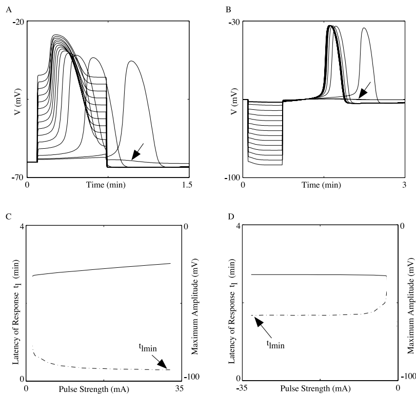
FIGURE 6 Latencies and amplitudes of pulse-induced responses. The responses and voltage dependence of the latencies to depolarizing (A and C) and hyperpolarizing (B and D) current injections. Examples of responses to depolarizing (A) and hyperpolarizing (B) pulses. Arrows denote subthreshold responses. The latencies of the responses decreased with absolute pulse amplitudes and approached minimum values, dashed-dot lines in C and D. Note the larger minimum latency in case of hyperpolarizing pulses. Pulse-induced slow wave amplitudes increased with pulse strength for depolarizing pulses while they remained constant in response to hyperpolarizing pulses, solid lines in C and D, respectively. Parameter values same as Fig. 2 except \beta = 0.7 \mu\text{M} .
