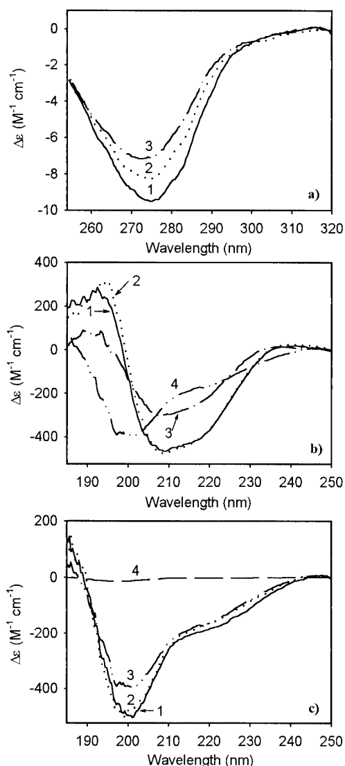
FIGURE 3 Comparison between the CD spectra of RNase A, RNase S, and S protein. (a) Near-UV CD: RNase A at 5°C (trace 1, —); RNase S at 4°C (trace 2, .....); and S protein at 5°C (trace 3, - - -). (b) Far-UV CD: RNase A at 5°C (trace 1, —); RNase S at 4°C (trace 2, .....); S protein at 5°C (trace 3, - - -), and S protein at 58°C (trace 4, - - -). (c) Denatured state spectra of RNase A at 78°C (trace 1, —); RNase S at 63°C (trace 2, .....); S protein at 58°C (trace 3, - - -); and S peptide at 58°C (trace 4, - - -). All the spectra are expressed as \Delta\epsilon ( M^{-1} \text{ cm}^{-1} ), where the molarity M refers to the molarity of the protein.
