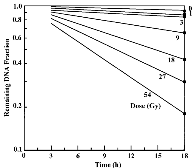
FIGURE 1 Decrease of Q_R with time for several experimental radiation exposures. The lines are based on the “smoothed” experimental values of Q_R(18) marked on the right edge (see Fig. 2).
