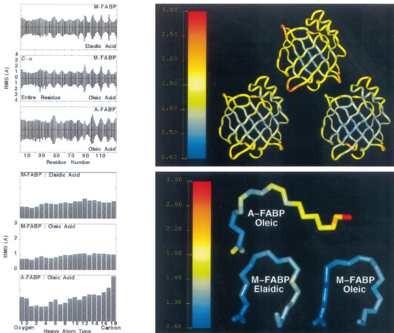
FIGURE 2 (A) RMS deviations from the trajectory averaged structure. Top two panels , M-FABP; bottom , A-FABP. The top of each panel represents C- \alpha deviations, and the bottom deviations are for all heavy atoms. In all cases, the x axis represents the residue number. Larger deviations are seen for the turns, compared to smaller deviations for \beta -sheets. The overall RMS deviations are small, indicative of a well-defined trajectory. (B) Mapping of the RMS deviations onto a color representation. The scale runs from blue to dark red (0–3 Å). This emphasizes the differences between the turns and \beta -sheets. (C) Fatty acid RMS deviations. The x axis moves along the heavy atoms of the ligand from the oxygens of the headgroup to the terminal methyl group. (D) Color mapping of the RMS deviations seen in C. The scale runs from blue to red (0.6–3.0 Å).
