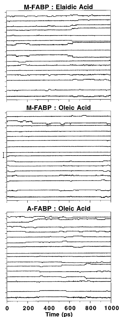
FIGURE 4 Time series of ligand dihedral angles. The bottom trace is from the headgroup, and the top trace is for the end of the alkane chain. Each trace was shifted by 360^\circ to make it possible to present all of the time series in a single figure. A 720^\circ scale bar is provided for the magnitude of changes in each trace. Tables 1–3 should be consulted for the numbers of transitions and observed pairs of dihedral changes.
