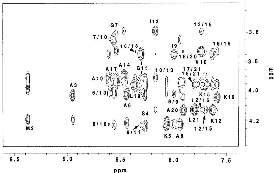
FIGURE 2 The fingerprint region of the two-dimensional homonuclear 1 H NOESY spectrum of PGLa in DPC micelles. The assignments of the intraresidue C α H-NH interresidue cross-peaks indicative of α-helical secondary structure are labeled.
