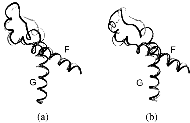
FIGURE 8 Motion of the FG loop. The coordinates of (a), the final CYP2A4 model ( dark ), and (b), the final CYP2A4/T model ( dark ), were superimposed onto the coordinates of CYP2A4 ( light ) early in the simulation. Helices F, G and the conserved core were used for the alignment. The FG loops exhibit moderate fluctuations in both cases.
