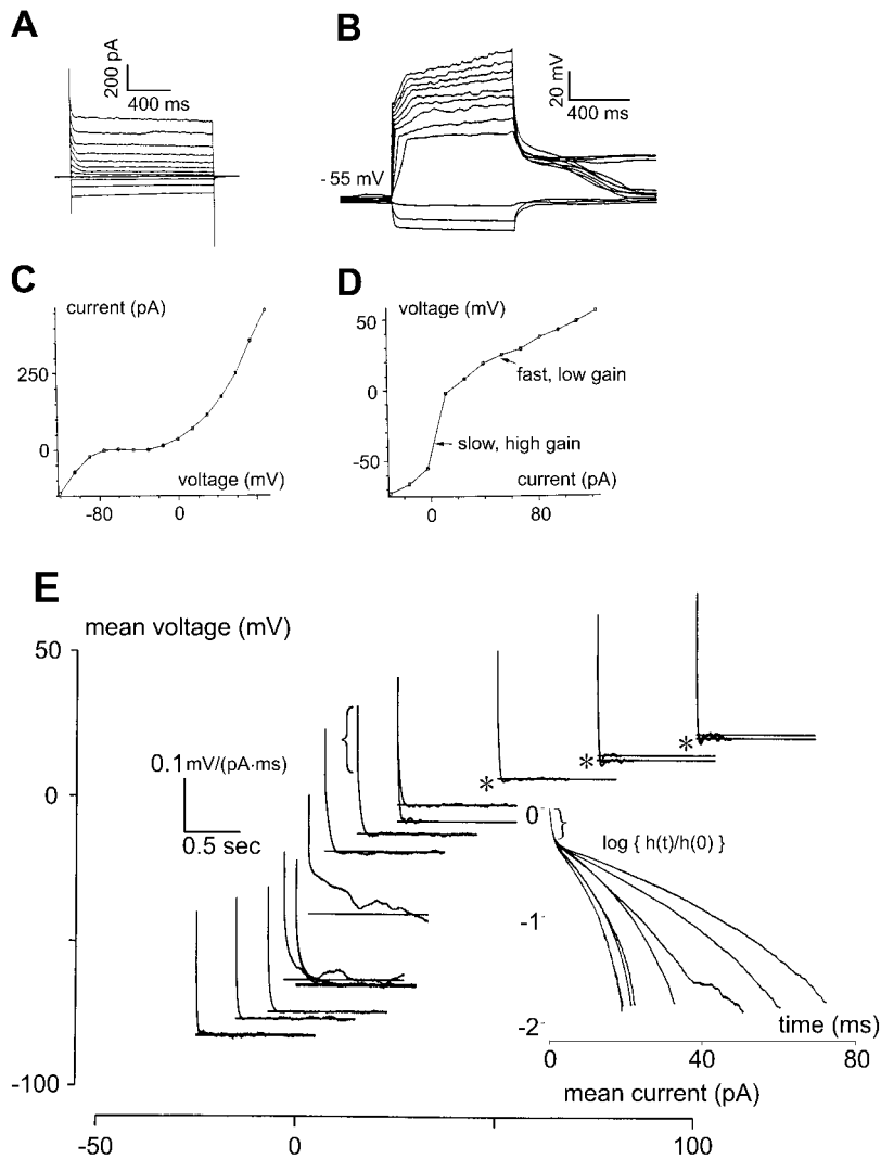
FIGURE 1 Membrane currents and intrinsic dynamics of bipolar cell. All recordings in solution A. (A) Current responses of a bipolar cell to voltage-clamp pulses ranging from -120 to 90 mV, in 15 -mV increments. An outward current was activated at membrane voltages > -30 mV and a prominent hyperpolarization-activated, inwardly rectifying current at membrane voltages < -50 mV. (B) Voltage responses of the bipolar cell to current-clamp pulses ranging from -30 to 124 pA, in 14 -pA increments. (C) Current-voltage relationship obtained from the current responses at the end of each of the voltage-clamp pulses shown in A. (D) Voltage-current relationship obtained from the voltage responses at the end of each of the current-clamp pulses shown in panel B. Note both outward and inward rectifications. (E) Effective impulse responses obtained by the m-sequence method and plotted in the (I,V) plane (as described in Methods). For depolarizing mean currents, the impulse response is rapidly attenuated, and also contains undershoots (asterisks). Consistent with the presence of the hyperpolarization-activated current in panel A, for hyperpolarizing mean currents ( -7 pA, -15 pA, -25 pA), membrane voltage shows inward rectification as evidenced by an attenuation of the impulse response. Impulse responses are also speeded up, due to the inwardly rectifying current, but there is no undershoot. (E, inset) Semilogarithmic plots of the impulse responses for depolarizing mean currents ( 15 pA, 25 pA, 50 pA, 75 pA, and 100 pA). The faster impulse response curves correspond to the more depolarizing mean currents. All impulse responses are convex, indicating that their declining phase is faster than that of exponential decline (which would be a straight line). The initial segments of all impulse responses reflect the series resistance of the recording pipette (indicated by brackets).
