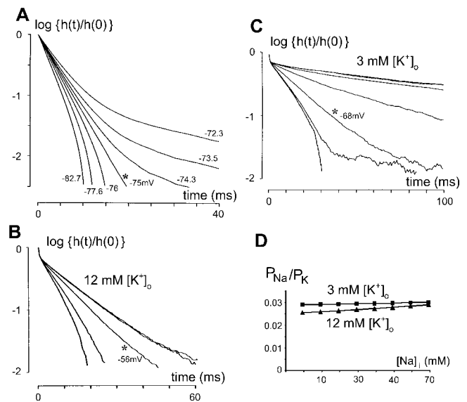
FIGURE 4 Estimating the reversal potential of a hyperpolarization-activated channel from a family of impulse responses. (A) Computer simulation demonstrating the validity of the method for estimating the reversal potential of hyperpolarization-activated channel. Parameters of the model bipolar neuron for the simulation are listed in Table 2. The hyperpolarization-activated channel has a reversal potential of E_h = -75 mV. The impulse responses above and below the known reversal potential ( -75 mV) are calculated as described in Methods and are plotted on the semilogarithmic scale. All the curves emanate from a common point and, in clockwise direction, these curves correspond to progressively more negative membrane voltage (in mV, -72.3 , -73.5 , -74.3 , -75.0 , -75.9 , -77.6 , and -82.7 ). At membrane voltages >-75 mV, the impulse response is concave; at voltages <-75 mV, impulse response is convex. Note that a transition between the two behaviors occurs precisely at the membrane potential equal to the reversal potential E_h -75 mV, at which the slope of the impulse response becomes a straight line ( asterisk ). (B) The method in panel A applied to the impulse responses for mean currents of 0 pA, 0 pA (repeated, two nearly overlapping curves), -3 pA, -15 pA, -25 pA, recorded from a bipolar cell in solution C (12 mM [K^+]_o ). The impulse response is concave (capacitive) for 0 pA and turns convex (inductive) between -3 pA and -15 pA. The membrane potential at the transition ( asterisk ), \sim -56 mV, is read from the V-I curve (not shown) at the point corresponding to -3 pA, and taken as an estimate of the reversal potential of the hyperpolarization-activated channel. (C) The method in panel A applied to the impulse responses for mean currents of 0 pA, 0 pA (repeated, two nearly overlapping curves), -3 pA, -7 pA, -15 pA, -25 pA (repeated), recorded from another bipolar cell in solution A (3 mM [K^+]_o ). The impulse response is concave (capacitive) for 0 pA, -3 pA, -7 pA, and turns convex (inductive) between -15 pA and -25 pA. The membrane potential at the transition ( asterisk ), \sim -68 mV, is read from the V-I curve (not shown) at -15 pA and taken as an estimate for the reversal potential of the hyperpolarization-activated channel. Note the convexity of the two traces for -25 pA is judged from the smooth portion of the curves at time <30 ms. The trace to the right contains much noise and has an amplitude that has decreased by more than one order of magnitude at times >40 ms. The portion corrupted by noise was ignored in the analysis of curvature. (D) The permeability ratio for Na^+ vs. K^+ ( P_{Na^+}/P_{K^+} ) for a range of [Na^+]_i (3–70 mM) is calculated as described in text. The average of the 14 reversal potentials of the hyperpolarization-activated channel under 3 mM [K^+]_o was used for estimating P_{Na^+}/P_{K^+} at that ionic condition. Similarly, average of 16 reversal potentials was used for P_{Na^+}/P_{K^+} estimation for 12 mM [K^+]_o condition.
