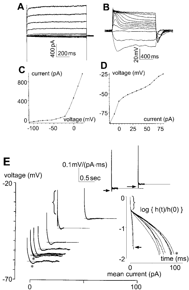
FIGURE 5 Membrane currents and intrinsic dynamics of the rod photoreceptor. All recordings in solution B (0.75 mM K^+ ). (A) Current responses of a rod photoreceptor to voltage-clamp pulses ranging from -110 to 22 mV, in 11 -mV increments. The large outward currents, presumably carried by K^+ , contain only a delayed-rectifierlike component. Slowly activated, small, but still distinguishable, currents are seen for voltages ranging from -30 mV to -100 mV. (B) Voltage responses of the rod photoreceptor to current-clamp pulses ranging from -16 to 80 pA, in 8 -pA increments. The voltage responses show slow overshoots for a broad range of current steps. (C) Current-voltage relationship, obtained from the current responses at the end of each of the voltage-clamp pulses shown in A. (D) Voltage-current relationship, obtained from the voltage responses at the end of each of the current-clamp pulses shown in B. (E) Effective impulse responses obtained as described in Methods. The impulse responses have undershoots in two ranges of membrane voltage: slow undershoots (asterisks) over a broad range near the resting potential, probably due to the I_h channel; fast undershoots (arrows) with marked depolarization, probably due to the delayed-rectifier K^+ channel. (E, inset) All the impulse responses in panel E are plotted on a semilogarithmic scale. All impulse responses are convex. Two impulse responses (arrows), much faster than the others, correspond to mean currents 75 and 100 pA, presumably due to the outward delayed-rectifier K^+ conductance. The initial segments of impulse responses reflect series resistance of the recording pipette (indicated by brackets).
