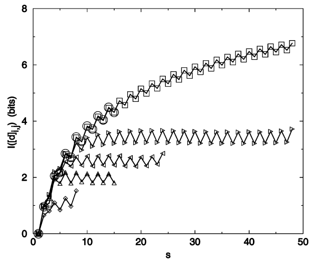
FIGURE 16 Mean information content for Hamilton square walks as a function of sequence separation for single distance constraints ( N = 9, 16, 25, 49 ), a full enumeration ensemble (FE) ( N = 16 ) and a stochastic, nonexhaustive ensemble of unconstrained conformations (FES) ( N = 49 ). \circ : 16-mer FE unit; \square : 49-mer FES; \diamond : 9-mer HW; \triangle : 16-mer HW; \triangleleft : 25-mer HW; \triangleright : 49-mer HW.
