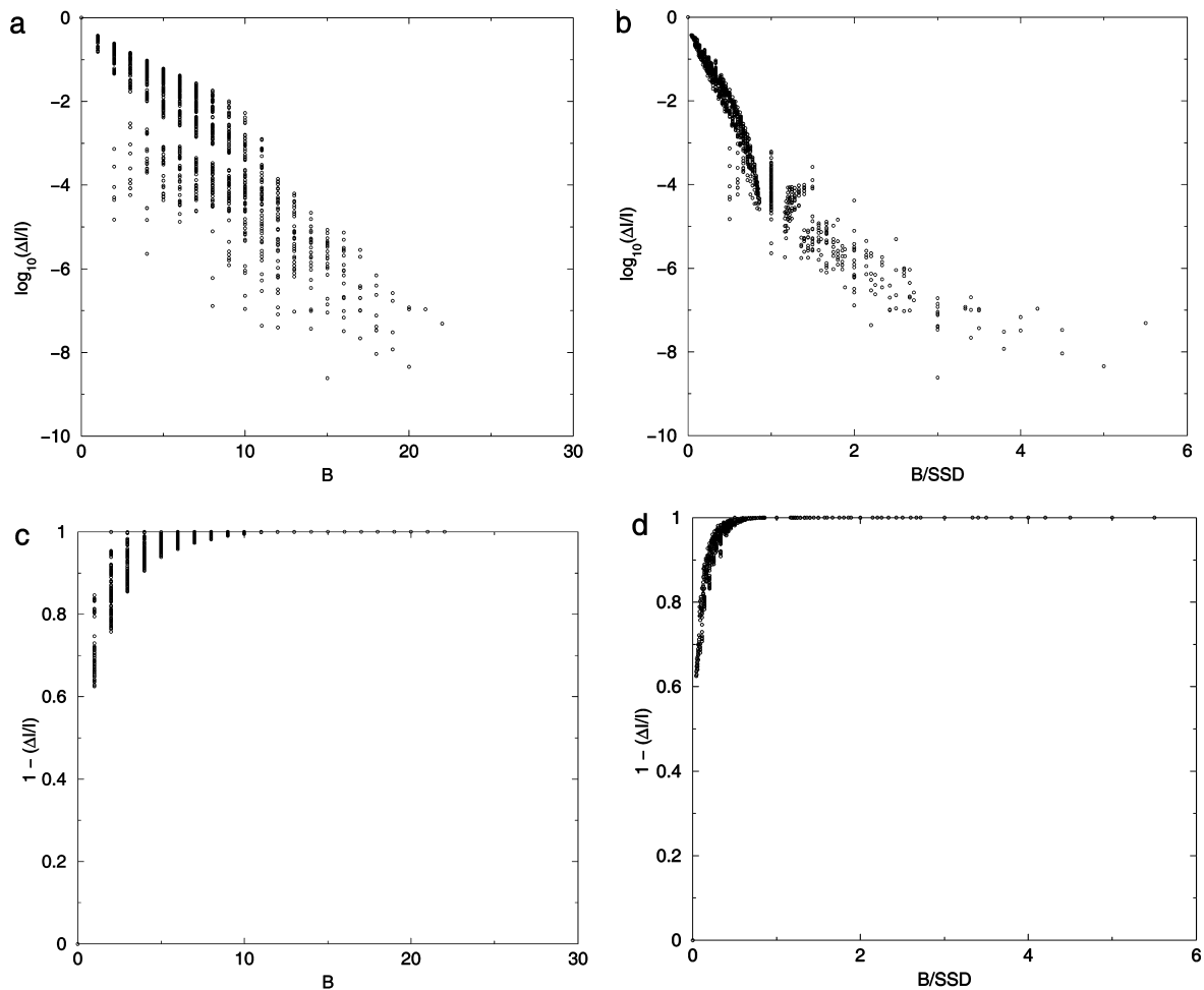
FIGURE 5 Relative information loss, \Delta I/I , for all pairs of distances, shown on a \log_{10} scale, calculated by Eq.14 as a function of transformations of the distance element distances. (a) The x axis is the block element identity distance, B , equal to |i - i'| + |j - j'| . (b) The x axis is B/SSD , where SSD = (s_{i,j} + s_{i',j'}) . (c) Plots (1 - \Delta I/I) versus B . (d) Plots (1 - \Delta I/I) vs. B/SSD .
