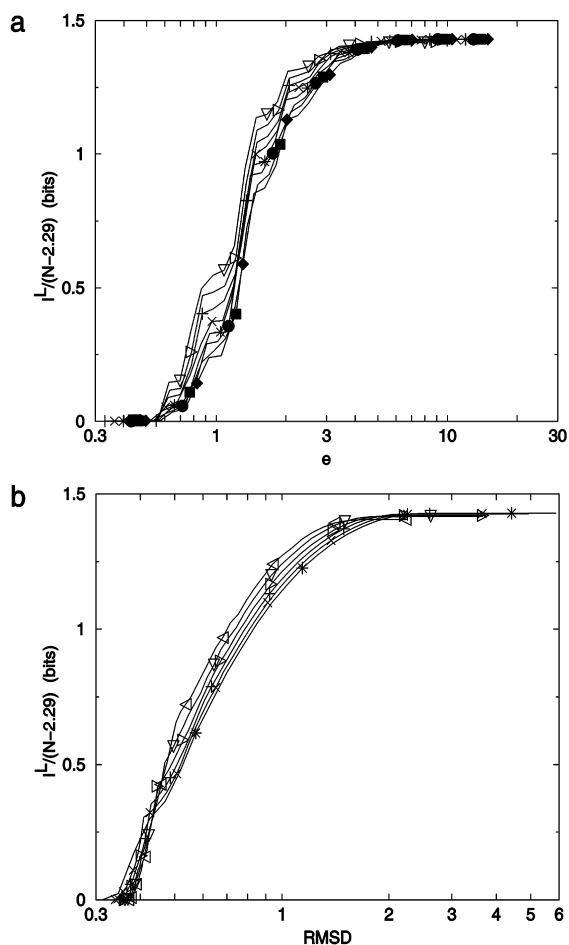
FIGURE 20 Information loss per degree of freedom for full enumeration, for N = 7 ( \nabla ), 8 ( \nabla ), 9 ( \triangleright ), 10 ( + ), 11 ( \times ), 12 ( * ), 13 ( \bullet ), 14 ( \blacksquare ), 15 ( \blacklozenge ). The factor (N - 2.29) comes from I^s = 1.43(N - 2.29) , a recasting of the self-avoiding walk equation for W(N) in Table 3. (a) Plotted against e . (b) Plotted against coordinate RMSD.
