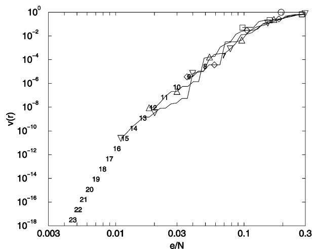
FIGURE 14 Conformational indistinguishability. \nu(r) is plotted as a function of the relative uncertainty, r = e/N . The limiting threshold noise levels for ensembles N = 7 - 23 are given by ensemble identity, N , and are placed at x = \{[(N - 3)^2 + 4]^{1/2} - (N - 3)\}/N , y = 2/[W \times (W - 1)] which are the limiting relative noise levels and inverse of total number of conformational pairs, respectively. \circ : 3-mer; \square : 6-mer; \diamond : 9-mer; \triangle : 12-mer; \nabla : 15-mer; 7-23: Limiting errors for 7-23 mers.
