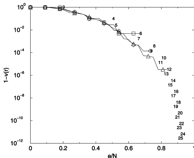
FIGURE 13 Conformational distinguishability. The fraction of distinguishable conformational pairs compared to the total number of conformational pairs, equal to 1 - \nu(r) , (see text) is plotted as a function of the relative noise, equal to r = e/N . \circ : 3-mer; \triangle : 6-mer; \triangleright : 9-mer; * : 12-mer; \circ : 13-mer.
