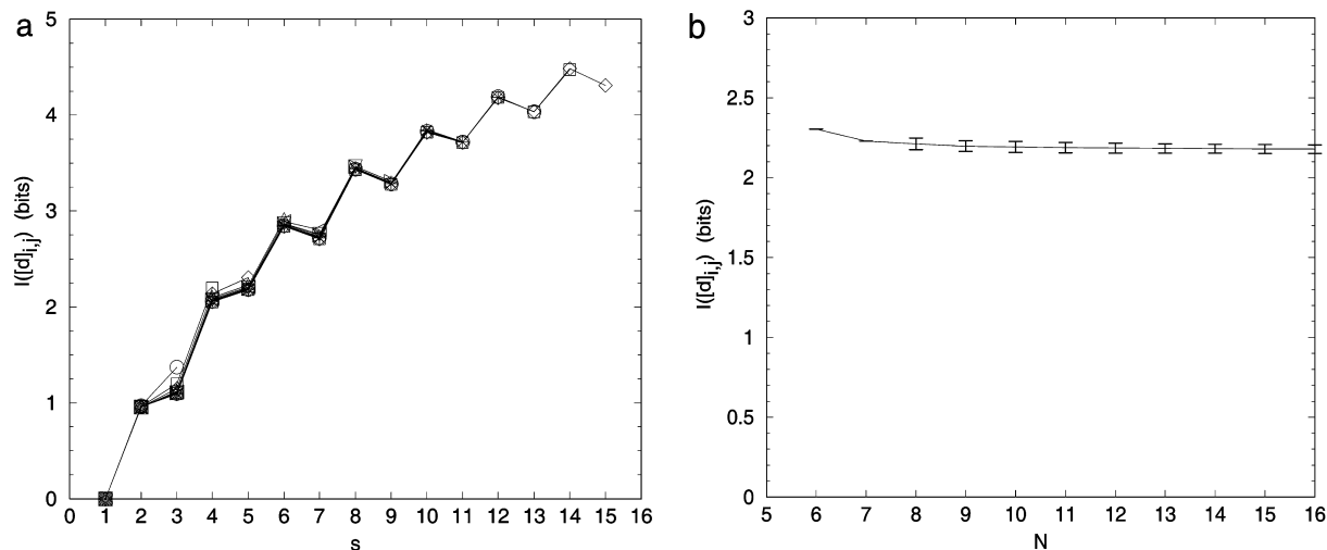
FIGURE 3 Information content by sequence separation. (a) Mean I([d]_{i,j}) as a function of s_{i,j} , for single distance elements [d]_{i,j} , plotted for exhaustive ensembles of N = 4 to N = 16 . (b) Independence of information content on chain length or chain position for fixed s_{i,j} = 5 .
