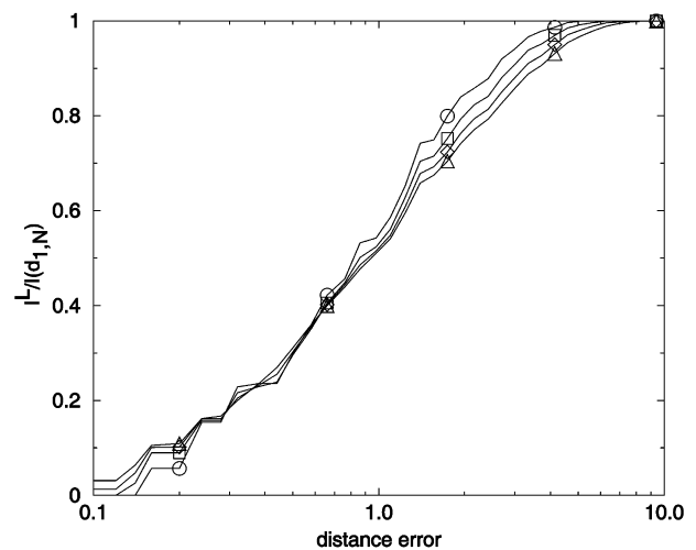
FIGURE 19 Relative information loss for [d]_{1,N} , full enumeration ensemble, for N = 9 ( \circ ), 11 ( \square ), 13 ( \diamond ), 15 ( \triangle ).
