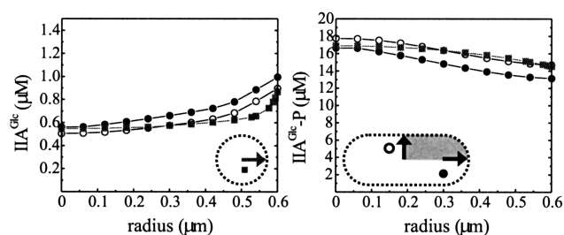
FIGURE 5 The concentration distribution of nonphosphorylated ( left ) and phosphorylated IIA Glc ( right ) in a spherical cell with radius 0.6 \mu\text{m} ( squares ), and in a rod-like cell with length 3 \mu\text{m} . The distribution in the latter is represented along two lines of length 0.6 \mu\text{m} perpendicular to the membrane boundary. These lines represent the two extremes found in the rod, i.e., through the center of the cylindrical part ( open circles ) and the spherical part ( closed circles ), respectively. The arrows in the insets represent the direction of the lines. The metabolite concentrations were as depicted in Table 1.
