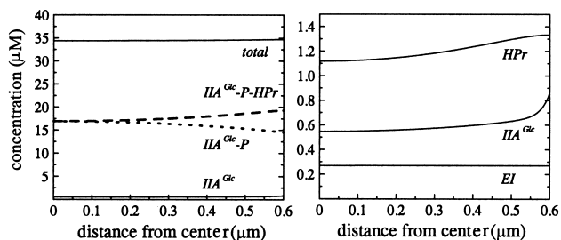
FIGURE 2 The concentration distribution of the IIA Glc -related ( left panel ) and nonphosphorylated cytoplasmic enzyme species ( right panel ) in a cell with radius 0.6 \mu\text{m} in the presence of both PEP ( 2.8 \text{mM} ) and glucose ( 500 \mu\text{M} ).
