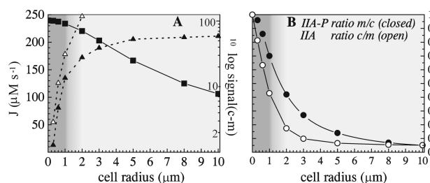
FIGURE 3 Cell size affects flux and concentration gradients. ( A ) Flux through the PTS ( left ordinate, squares ), and the difference in signal concentration between cell center and inner membrane as a function of cell radius ( right ordinate, triangles ). The open triangles represent a rough estimate based on Eq. 7 and the calculated flux, and the closed triangles represent the result of the precise calculation using Eq. 6 (note that the scale is logarithmic). ( B ) The concentration ratio of phosphorylated IIA Glc ( closed circles, membrane/center ) and of nonphosphorylated IIA Glc ( open circles, center/membrane ). The dark gray area is relevant for bacterial dimensions, the light gray area for eukaryotic cells.
