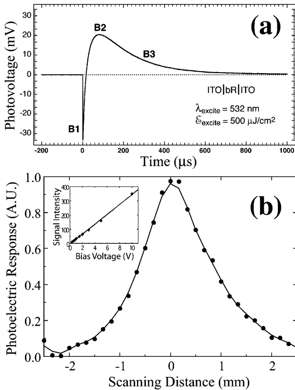
FIGURE 3 (a) Measured photoelectric response characteristics of dried film of BR oriented between two ITO plates. The fast (B1) and slow (B2 and B3) components are associated with both structural changes in the protein as well as net translocation of the proton. The rise and decay time of B1 could not be accurately measured due to the limited bandwidth of the measurement system. The photoelectric response of the BR film as a function of scanning distance is shown in b . The pump and probe beams were focused during the mapping process to achieve a spatial resolution of 300 \mu\text{m} . The inset indicates that, in the electro-optic sampling measurement, the detected light intensity is directly proportional to the electric field inside the BGO crystal.
