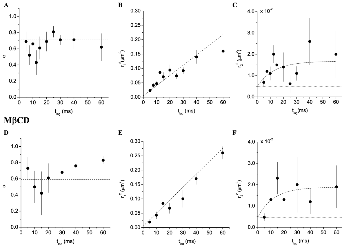
FIGURE 4 Results obtained from the square displacement distribution analysis of data taken on 3T3-A14 cells at 37°C after drug treatment. The fit results obtained for DMSO-treated cells (A–C) and untreated cells (D–F) are shown for comparison as dashed lines, results from the fits are given in Table 1. (A–C) Fraction (A) and mean-squared displacement of the fast (B) and the slow (C) fraction after treatment with 0.5 \mu\text{M} latrunculin B for 30 min. (D–F) Fraction (D), and mean-squared displacement of the fast (E) and the slow (F) fraction after treatment with 5 mM methyl- \beta -cyclodextrin for 1 h. The dotted lines in C and F represent the offset due to the limited positional accuracy (see Materials and Methods); they have been omitted in B and E for clarity.
