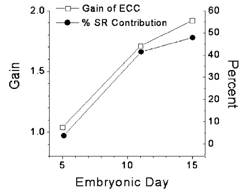
FIGURE 6 Computed gain factor for CICR and percent contribution to the Ca^{2+} transient from the SR are illustrated together for comparison. The values were calculated using the Ca^{2+} buffer power and the data from the field-stimulated Ca^{2+} transients illustrated in Fig. 1 as detailed in the text. The increase in gain and SR contribution parallels the structural development of SR junctions as demonstrated in Protasi et al. (1996; compare this Fig. 6 with their Fig. 4).
