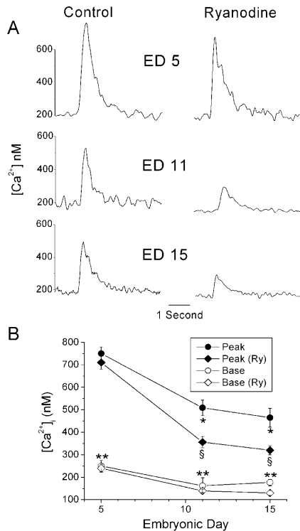
FIGURE 1 The effect of ryanodine ( Ry ) on electrically stimulated intracellular \text{Ca}^{2+} transients during development. (A) Examples of \text{Ca}^{2+} transients illustrating the effects before and after the addition of 100 \mu\text{M} ryanodine. Note that \text{Ca}^{2+} transients are larger at ED5 compared to ED11 and 15, whereas the effect of ryanodine is smaller. (B) Graphical representation illustrating that most of the decline in the magnitude of \text{Ca}^{2+} transients as well as the largest increase in the effect of ryanodine occurs between ED5 and 11. Peak indicates the peak magnitude of the \text{Ca}^{2+} transient and base indicates the baseline \text{Ca}^{2+} level after decay of the \text{Ca}^{2+} transient and just before the beginning of the next transient. N = 7 myocytes for each of the three ages. The data points represent 2–3 experiments per age with 2–4 myocytes per experiment. Error bars indicate mean \pm SE. Single asterisk (*) indicates statistical significance when comparing either ED11 or 15 with ED5. Section symbol (§) indicates significant reduction in the peak after ryanodine treatment in paired comparisons with the student's t -test. Double asterisk (**) indicates that the baseline was significantly less after ryanodine treatment when compared using the paired student's t -test.
