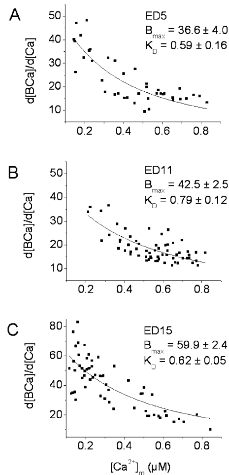
FIGURE 5 Cytosolic Ca buffering. [\text{Ca}^{2+}]_{\text{m}} and d[\text{BCa}]/d[\text{Ca}] were calculated and fitted to Eq. 2 as described in the text. The K_{\text{D}} and B_{\text{max}} (mean \pm SE) for each age are shown in A–C, and were determined by fitting the data set for each myocyte individually. The cumulative data for each age is shown in the graphs. Note that d[\text{BCa}]/d[\text{Ca}] is the chord buffer power for any given level of cytosolic-free \text{Ca}^{2+} . N = 5, 8, \text{ and } 8 , for ED5, 11, and 15, respectively. The data are from four experiments for each age and 1–3 cells per experiment. Units of B_{\text{max}} are in \mu\text{M}/\text{liter} cell water and K_{\text{D}} values are in \mu\text{M} .
