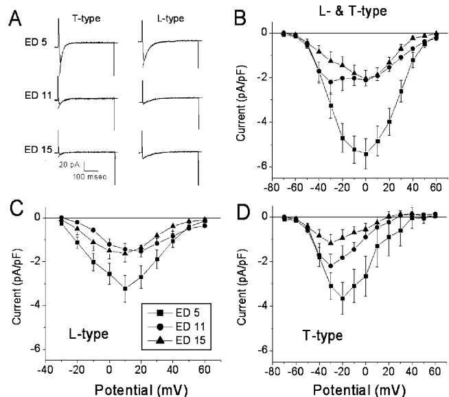
FIGURE 2 Examples of L- and T-type \text{Ca}^{2+} currents and current-voltage (I-V) relationships from ED5, 11, and 15. (A) Example of current traces illustrating T-type \text{Ca}^{2+} current elicited from steps to -30 mV from the holding potential of -80 mV and L-type current from a step to +10 mV after a prepulse to -40 mV to inactivate the T-current. Note that the \text{Ca}^{2+} currents are largest at ED5. The overlying smooth curves illustrate the single-exponential fits to the decaying phase of the currents. (B) I-V curves elicited by voltage steps from a -80 -mV holding potential showing the peak values for inward \text{Ca}^{2+} currents. The biphasic I-V curve most noticeable at ED11 is due to the presence of T-type \text{Ca}^{2+} current which activates at a lower threshold compared to L-type current (see text). (C) I-V relationships for L-type \text{Ca}^{2+} current elicited after inactivation of T-type current with a 500-ms prepulse to -40 mV. (D) The I-V relationship for T-type current was determined by subtracting the values illustrated in C from those in B. N = 15 , 10, and 15 for ED5, 11, and 15, respectively, and 3–5 cells per experiment. Error bars indicate mean \pm SE.
