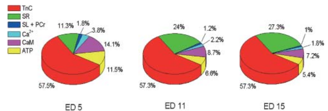
FIGURE 8 Graphical representation of the proportion of \text{Ca}^{2+} bound by the major cytoplasmic fast \text{Ca}^{2+} binding moieties at the peak of the intracellular \text{Ca}^{2+} transient at the three developmental ages. Note that TnC binds \sim 57\% of the \text{Ca}^{2+} at each age. The proportion of \text{Ca}^{2+} bound by the SR increases, and this is offset primarily by corresponding decreases in \text{Ca}^{2+} bound by calmodulin and ATP. \text{Ca}^{2+} binding to total sarcolemmal (SL) sites and to creatine phosphate (PCr) is small and has been combined in the figure.
