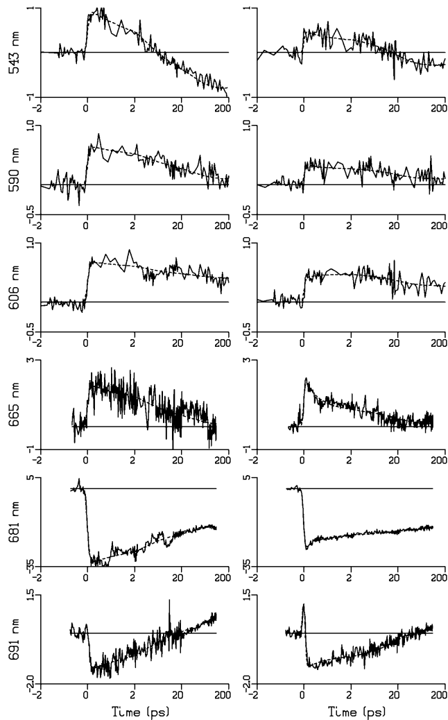
FIGURE 3 Kinetic traces ( solid ) and fits to the data ( dashed ) for untreated RC ( left ) and RC 1x ( right ) at representative wavelengths in the Q X and Q Y regions. Unit of \Delta A is mOD. The timescale is linear between -2 and 2 ps and logarithmic for later delays.
