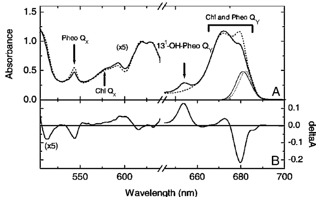
FIGURE 1 (A) The 6-K absorption spectra of the two types of RCs used for time-resolved absorption difference spectra: untreated RC (dotted) and RC_{1x} (solid). The wavelength profile of the pump laser beam for the measurements was similar to the ones shown here (thin lines) and had a maximum at 683 nm. (B) Absorption-difference spectrum associated with the exchange of H_B , calculated from the spectra in A. In both A and B, the signals below 640 nm are shown at 5 \times enlarged amplitude. (Adapted from Germano et al., 2001.)
