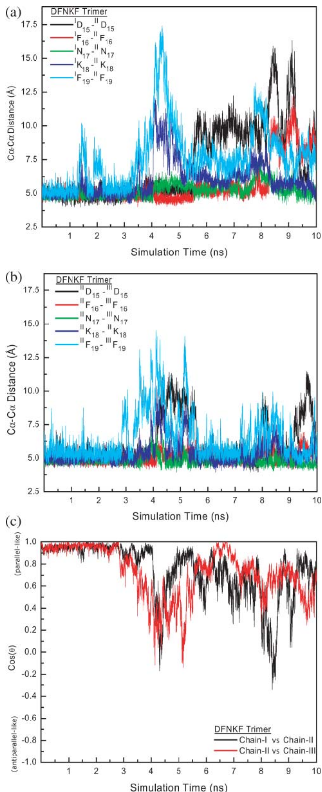
FIGURE 6 Structural characteristics (pairwise residue C \alpha -C \alpha distances and cross angle between chains) of the DFNKF trimer. (a) The pairwise residue C \alpha -C \alpha distances between chain-I and chain-II. (b) The pairwise residue C \alpha -C \alpha distances between chain-II and chain-III. (c) The time dependence of \cos(\theta) , the cross angle between the chains. The definition of
