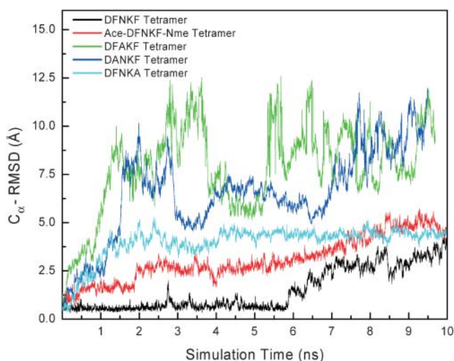
FIGURE 10 The C_{\alpha} -RMSD of four DF/NKF sequence variants and original DF/NKF tetramer as a function of time. The four sequence variants included one capped variant, Ace-DF/NKF-Nme tetramer, and three mutants, DFAKF, DANKF, and DF/NKA tetramers. The initial structures for all calculations were in the parallel arrangements. The C_{\alpha} -RMSDs were calculated from the corresponding energy minimized structures in parallel manners. The C_{\alpha} -RMSD of the original DF/NKF tetramer is also plotted for comparison. The C_{\alpha} -RMSDs are the indicators of the relative stabilities of the DF/NKF sequence variants from the original DF/NKF. The Ace-DF/NKF-Nme and DF/NKA tetramers are slightly less stable than the original DF/NKF tetramer. Comparing the C_{\alpha} -RMSDs of the DFAKF and DANKF with the original DF/NKF indicated that these mutants are relatively unstable.
