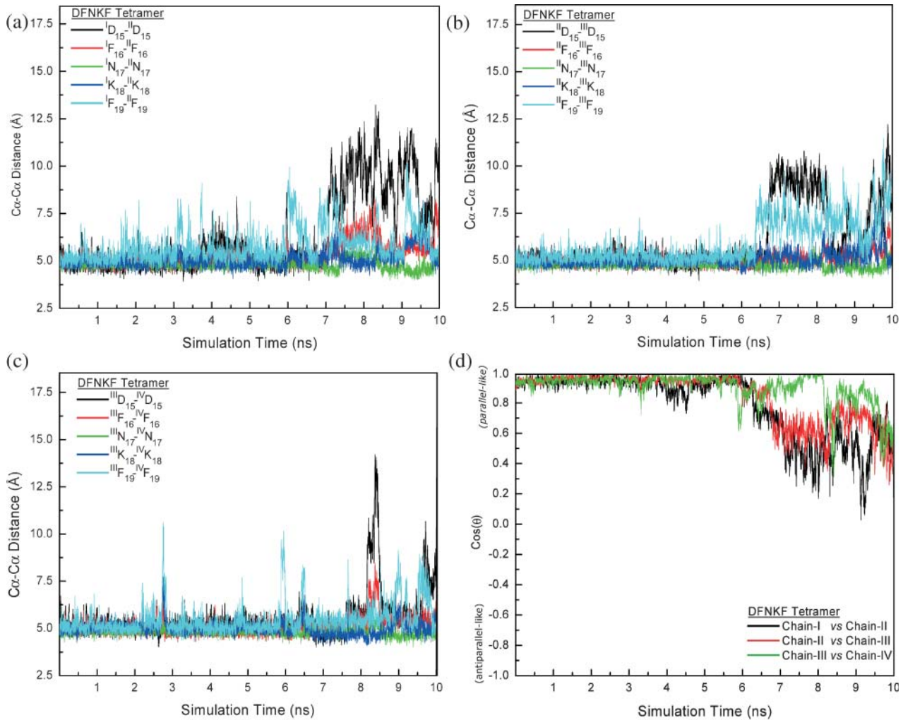
FIGURE 9 Structural characteristics (pairwise residue C_{\alpha} - C_{\alpha} distances and cross angle between chains) of the DFNKF tetramer. (a) The pairwise residue C_{\alpha} - C_{\alpha} distances between chain-I and chain-II. (b) The pairwise residue C_{\alpha} - C_{\alpha} distances between chain-II and chain-III. (c) The pairwise residue C_{\alpha} - C_{\alpha} distances between chain-III and chain-IV. (d) The time dependence of \cos(\theta) , the cross angle between the chains. The definition of \cos(\theta) is shown in Computational Methods. Only the cross angles between chain-I versus chain-II, chain-II versus chain-III, and chain-III versus chain-IV are shown. For comparison, the same scale is used as in the plots of the DFNKF trimer in Fig. 6. The fluctuations of the DFNKF tetramer are smaller compared to the DFNKF trimer results in Fig. 6. The structural characteristics of chain-III versus chain-IV are nearly in-register and parallel during the whole simulation. The Asp at the N-terminal and Phe residues at the C-terminal are relatively more flexible than other residues, similar to the observations in the dimer and trimer simulations.
