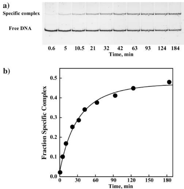
FIGURE 2 (a) A polyacrylamide gel illustrating the kinetics of specific Eco RI binding to the 360-bp DNA fragment in the presence of the TAATTC “star” sequence oligonucleotide. In the absence of oligonucleotide, specific sequence binding is complete within 5 min. The dissociation rate of Eco RI from the TAATTC oligonucleotide complex is determined from the time dependence. The gel mobility shift assay is used to monitor the gain of specific Eco RI-DNA complex. Eco RI (1.5 nM) was incubated for different times with a mixture of specific sequence DNA fragment (3 nM) and the TAATTC sequence oligonucleotide. The particular conditions used in this experiment were 90 mM NaCl, 3.95 Osm betaine glycine, 20 mM imidazole (pH 7.0), and 20°C. The TAATTC sequence oligonucleotide was present in 250-fold molar excess over the specific sequence fragment. (b) The fraction of the specific Eco RI-DNA fragment complex is shown plotted against time for the gel shown in panel a. The solid line is the best fit of Eq. 7 to the data. The dissociation rate constant k_4 for this complex was calculated as 2.4 \text{ min}^{-1} .
