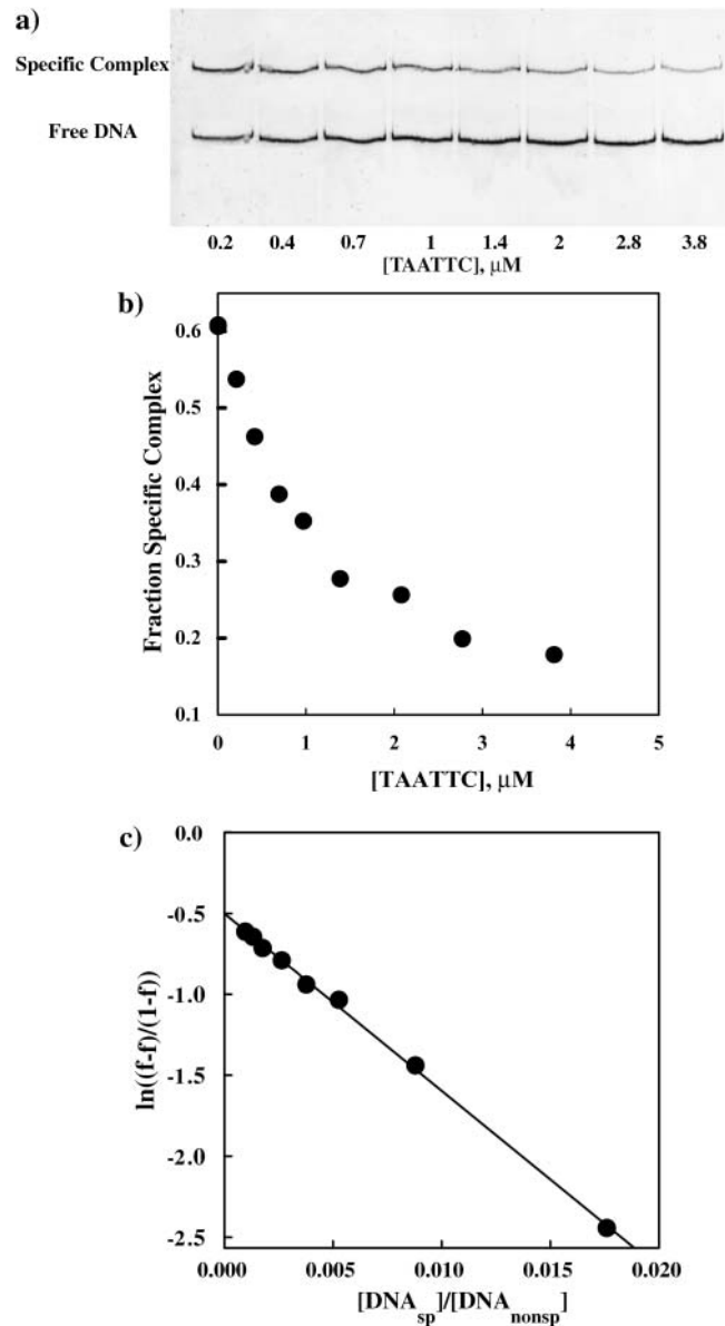
FIGURE 3 (a) The fraction of specific sequence complex formed after one hour incubation decreases as the concentration of noncognate oligonucleotide increases. Eco RI (1.5 nM) was incubated with specific sequence DNA fragment (3 nM) and varying concentrations of noncognate oligonucleotides in 75 mM NaCl, 20 mM imidazole (pH 7.0), 3.6 Osm betaine, and at 20°C. The gel mobility shift assay was used to monitor specific complex formation. (b) The dependence of the specific Eco RI-DNA complex fraction on TAATTC sequence oligonucleotide concentration for the gel shown in panel a. (c) The linear dependence of \ln((f-f)/(1-f)) on [DNA_{\text{sp}}]_{\text{tot}}/[DNA_{\text{nonsp}}]_{\text{tot}} confirms the concentration dependence predicted by Eq. 4. The dissociation rate constant, k_4 , of the TAATTC “star” sequence oligonucleotide complex can be calculated from the slope. For this particular experiment, k_4 is 0.86 \text{ min}^{-1} .
